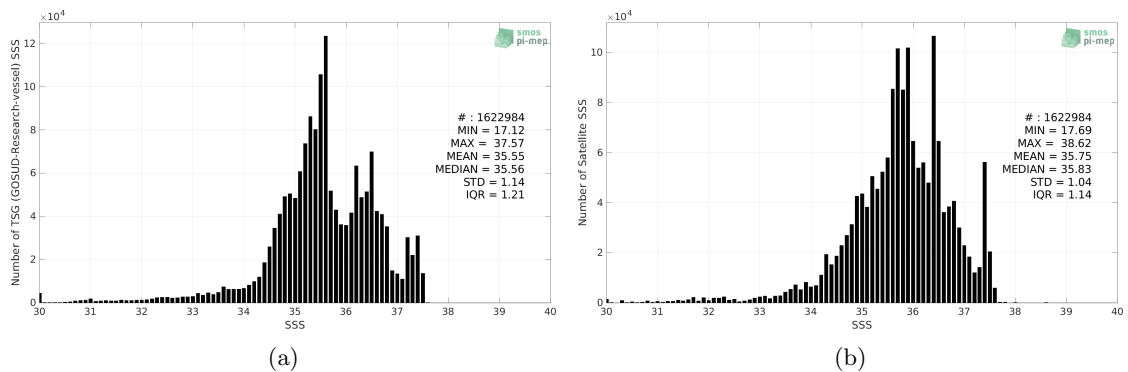
Figure 2: Histograms of SSS from TSG (GOSUD-Research-vessel) (a) and SMAP SSS L3 v5 - Monthly (RSS) (b) considering all match-up pairs per bins of 0.1 over the North Atlantic Ocean Pi-MEP region and for the full satellite product period.
