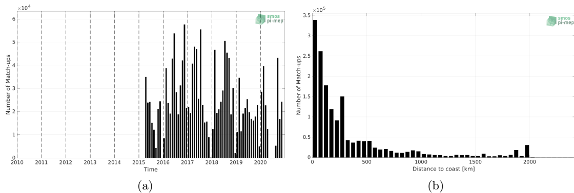
Figure 1: Number of match-ups between TSG (GOSUD-Research-vessel) and SMAP SSS L3 v5 - Monthly (RSS) SSS as a function of time (a) and as function of the distance to coast (b) over the North Atlantic Ocean Pi-MEP region and for the full satellite product period.
