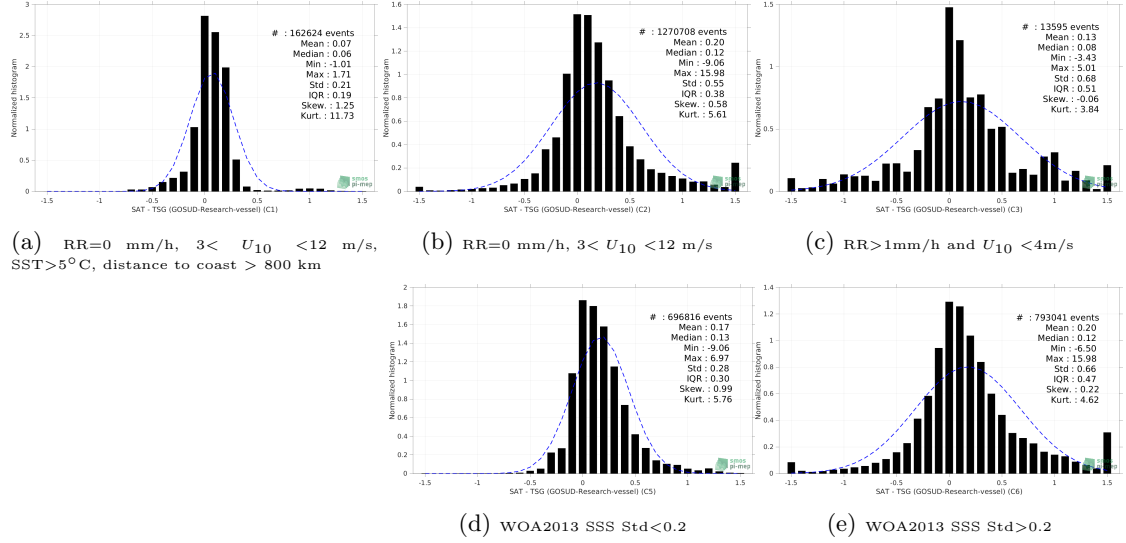
Figure 13: Normalized histogram of \Delta\text{SSS} (SMAP SSS L3 v5 - Monthly (RSS) - TSG (GOSUD-Research-vessel)) for 5 different subdatasets corresponding to: RR=0 mm/h, 3 < U_{10} < 12 m/s, SST>5°C, distance to coast > 800 km (a), RR=0 mm/h, 3 < U_{10} < 12 m/s (b), RR>1mm/h and U_{10} < 4 m/s (c), WOA2013 SSS Std<0.2 (d), WOA2013 SSS Std>0.2 (e).
