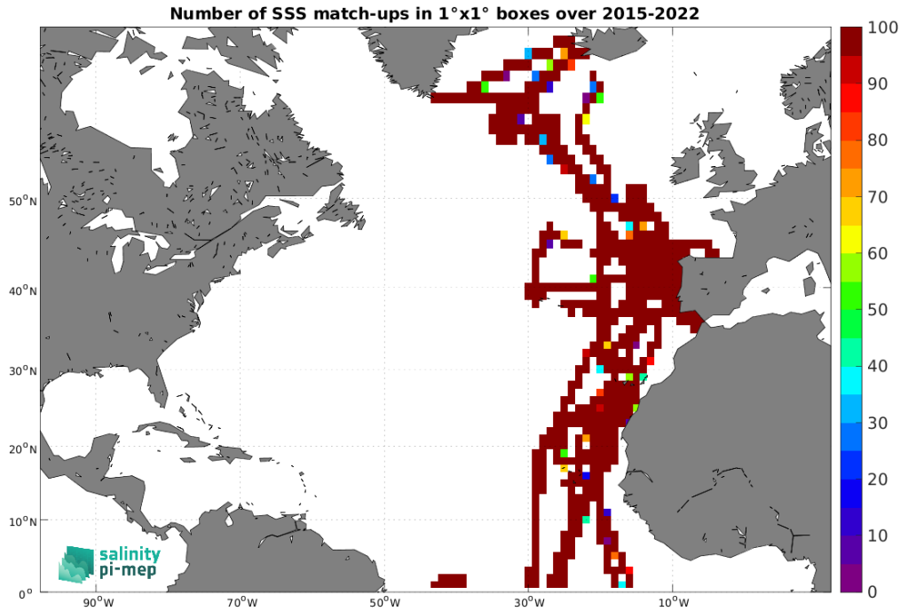
Figure 4: Number of SSS match-ups between TSG (CSIC-UTM) SSS and the SMAP SSS L3 v5 - Monthly (RSS) SSS product for the North Atlantic Ocean Pi-MEP region over 1^{\circ} \times 1^{\circ} boxes and for the full satellite product period.
