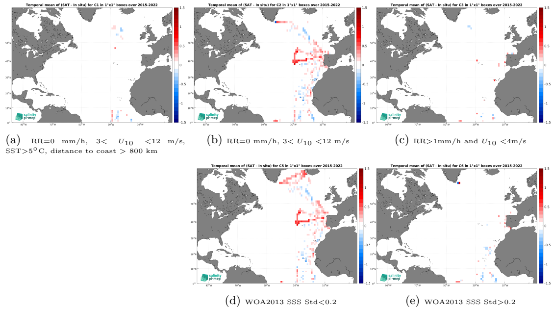
Figure 12: Temporal mean gridded over spatial boxes of size 1^\circ \times 1^\circ of \Delta\text{SSS} (SMAP SSS L3 v5 - Monthly (RSS) - TSG (CSIC-UTM)) for 5 different subdatasets corresponding to:RR=0 mm/h, 3 < U_{10} < 12 m/s, SST >5^\circ\text{C} , distance to coast > 800 km (a), RR=0 mm/h, 3 < U_{10} < 12 m/s (b), RR >1 mm/h and U_{10} < 4 m/s (c), WOA2013 SSS Std <0.2 (d), WOA2013 SSS Std >0.2 (e).
