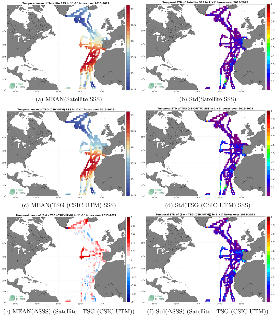
Figure 6: Temporal mean (left) and Std (right) of SSS from SMAP SSS L3 v5 - Monthly (RSS) (top), TSG (CSIC-UTM) (middle), and of \Delta SSS (Satellite - TSG (CSIC-UTM)). Only match-up pairs are used to generate these maps.
