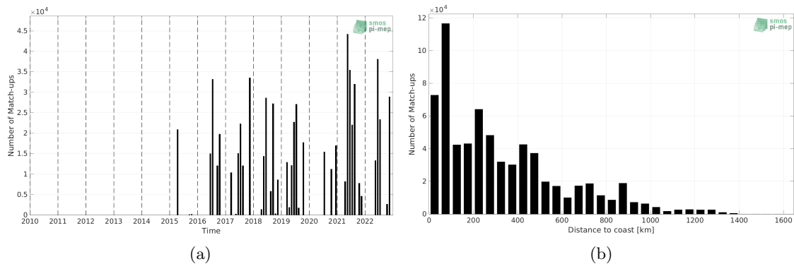
Figure 1: Number of match-ups between TSG (CSIC-UTM) and SMAP SSS L3 v5 - Monthly (RSS) SSS as a function of time (a) and as function of the distance to coast (b) over the North Atlantic Ocean Pi-MEP region and for the full satellite product period.
