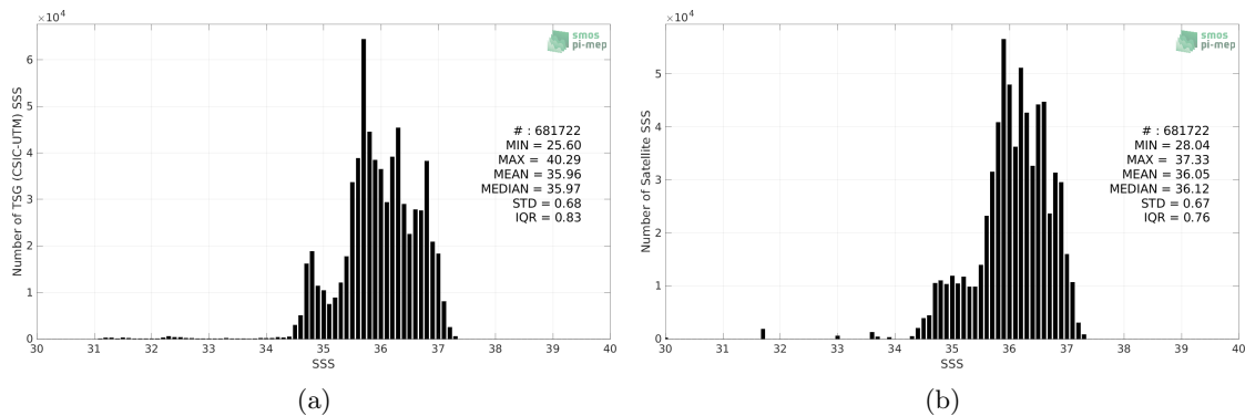
Figure 2: Histograms of SSS from TSG (CSIC-UTM) (a) and SMAP SSS L3 v5 - Monthly (RSS) (b) considering all match-up pairs per bins of 0.1 over the North Atlantic Ocean Pi-MEP region and for the full satellite product period.
