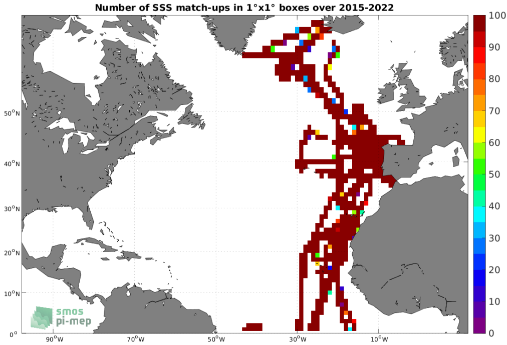
Figure 4: Number of SSS match-ups between TSG (CSIC-UTM) SSS and the SMAP SSS L3 v5 - Monthly (RSS) SSS product for the North Atlantic Ocean Pi-MEP region over 1^\circ \times 1^\circ boxes and for the full satellite product period.
