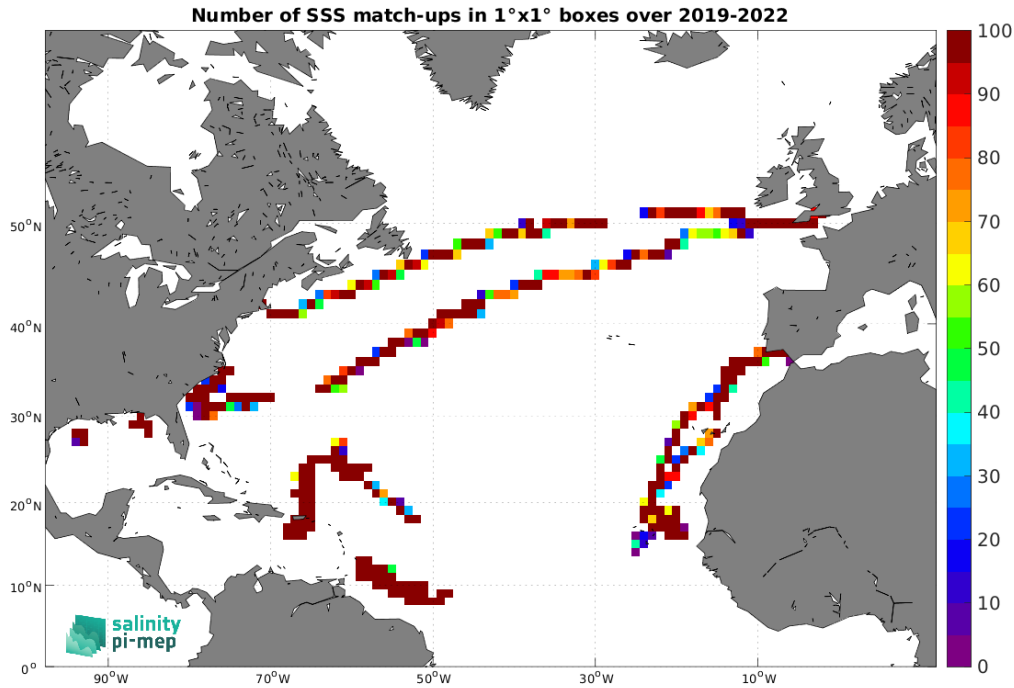
Figure 4: Number of SSS match-ups between Saildrone SSS and the SMAP SSS L3 v5 - Monthly (RSS) SSS product for the North Atlantic Ocean Pi-MEP region over 1^\circ \times 1^\circ boxes and for the full satellite product period.
