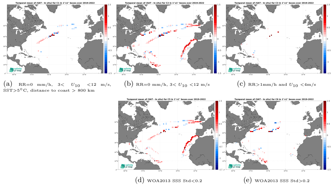
Figure 12: Temporal mean gridded over spatial boxes of size 1^\circ \times 1^\circ of \Delta\text{SSS} (SMAP SSS L3 v5 - Monthly (RSS) - Saildrone) for 5 different subdatasets corresponding to:RR=0 mm/h, 3 < U_{10} < 12 m/s, SST >5^\circ\text{C} , distance to coast > 800 km (a), RR=0 mm/h, 3 < U_{10} < 12 m/s (b), RR >1 mm/h and U_{10} < 4 m/s (c), WOA2013 SSS Std <0.2 (d), WOA2013 SSS Std >0.2 (e).
