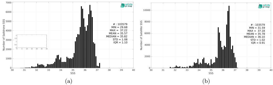
Figure 2: Histograms of SSS from Saildrone (a) and SMAP SSS L3 v5 - Monthly (RSS) (b) considering all match-up pairs per bins of 0.1 over the North Atlantic Ocean Pi-MEP region and for the full satellite product period.
