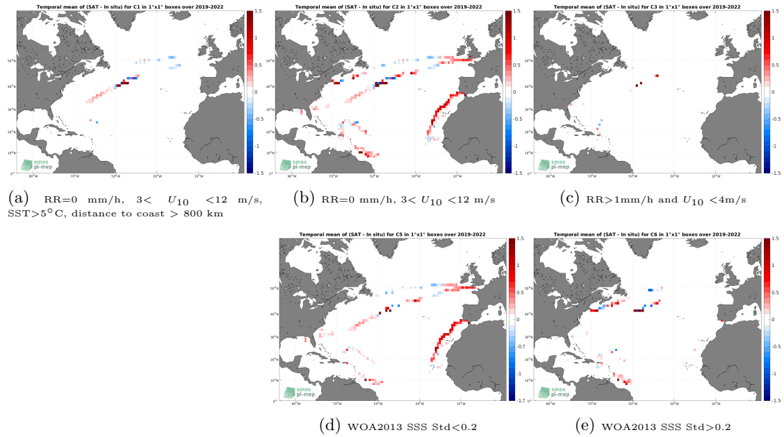
Figure 12: Temporal mean gridded over spatial boxes of size 1^\circ \times 1^\circ of \Delta SSS (SMAP SSS L3 v5 - Monthly (RSS) - Saildrone) for 5 different subdatasets corresponding to:RR=0 mm/h, 3 < U_{10} < 12 m/s, SST >5^\circ\text{C} , distance to coast > 800 km (a), RR=0 mm/h, 3 < U_{10} < 12 m/s (b), RR >1 mm/h and U_{10} < 4 m/s (c), WOA2013 SSS Std <0.2 (d), WOA2013 SSS Std >0.2 (e).
