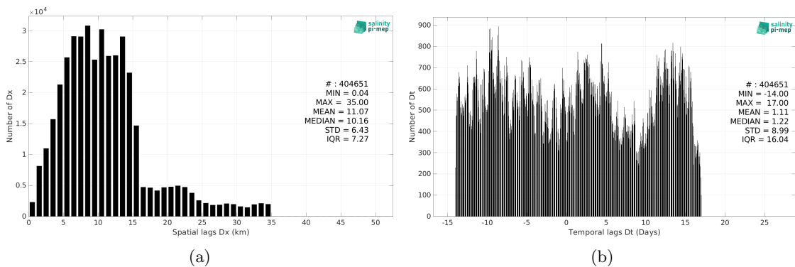
Figure 5: Histograms of the spatial (a) and temporal (b) lags between the location/time of the ICES measurement and the date of the corresponding SMAP SSS L3 v5 - Monthly (RSS) SSS pixel.
