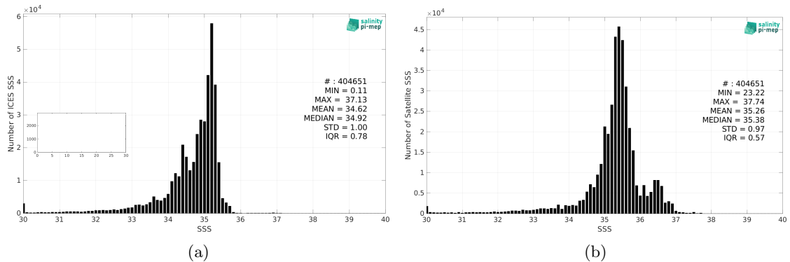
Figure 2: Histograms of SSS from ICES (a) and SMAP SSS L3 v5 - Monthly (RSS) (b) considering all match-up pairs per bins of 0.1 over the North Atlantic Ocean Pi-MEP region and for the full satellite product period.
