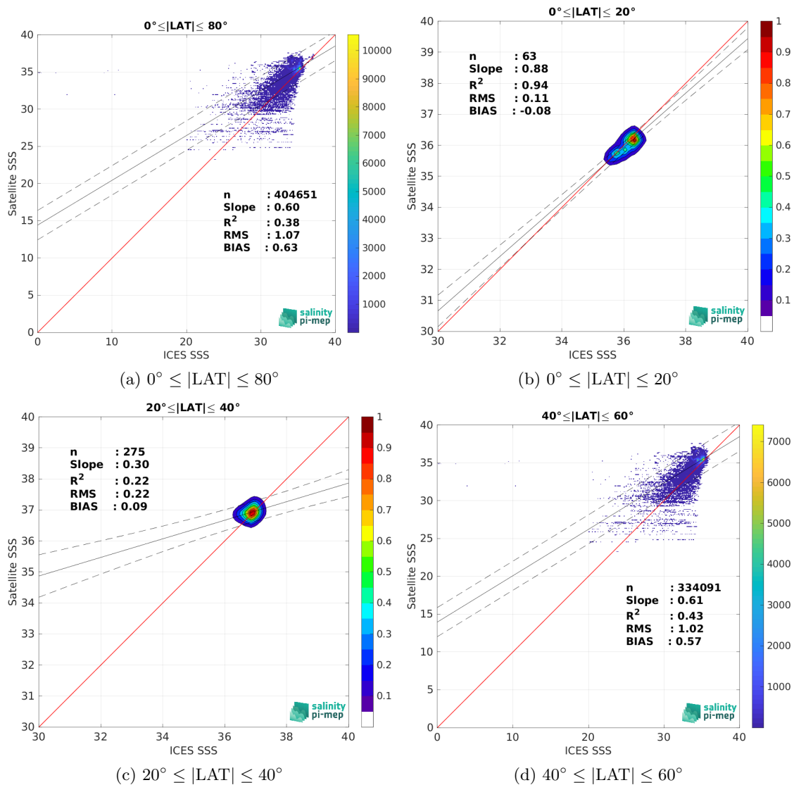
Figure 9: Contour maps of the concentration of SMAP SSS L3 v5 - Monthly (RSS) SSS (y-axis) versus ICES SSS (x-axis) at match-up pairs for different latitude bands. For each plot, the red line shows x=y . The black thin and dashed lines indicate a linear fit through the data cloud and the \pm 95\% confidence levels, respectively. The number match-up pairs n , the slope and R^2 coefficient of the linear fit, the root mean square (RMS) and the mean bias between satellite and in situ data are indicated for each latitude band in each plots.
