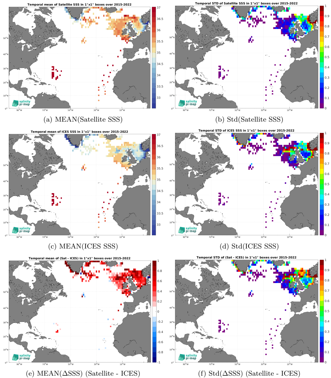
Figure 6: Temporal mean (left) and Std (right) of SSS from SMAP SSS L3 v5 - Monthly (RSS) (top), ICES (middle), and of \Delta SSS (Satellite - ICES). Only match-up pairs are used to generate these maps.
