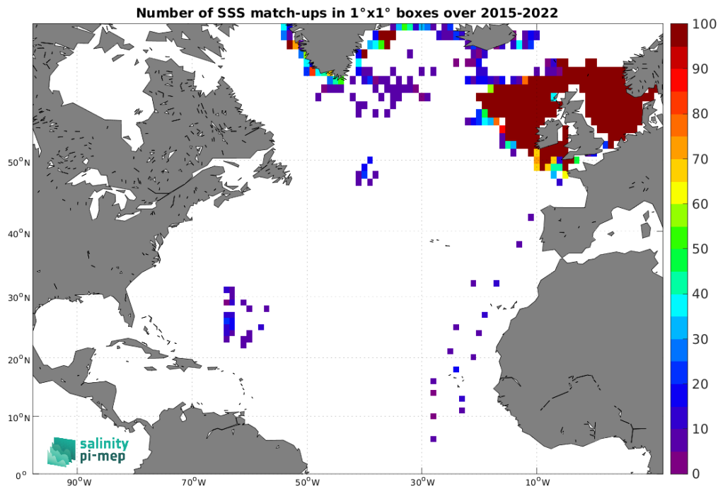
Figure 4: Number of SSS match-ups between ICES SSS and the SMAP SSS L3 v5 - Monthly (RSS) SSS product for the North Atlantic Ocean Pi-MEP region over 1^\circ \times 1^\circ boxes and for the full satellite product period.
