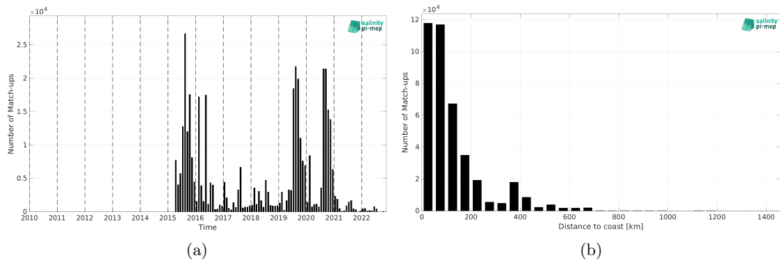
Figure 1: Number of match-ups between ICES and SMAP SSS L3 v5 - Monthly (RSS) SSS as a function of time (a) and as function of the distance to coast (b) over the North Atlantic Ocean Pi-MEP region and for the full satellite product period.
