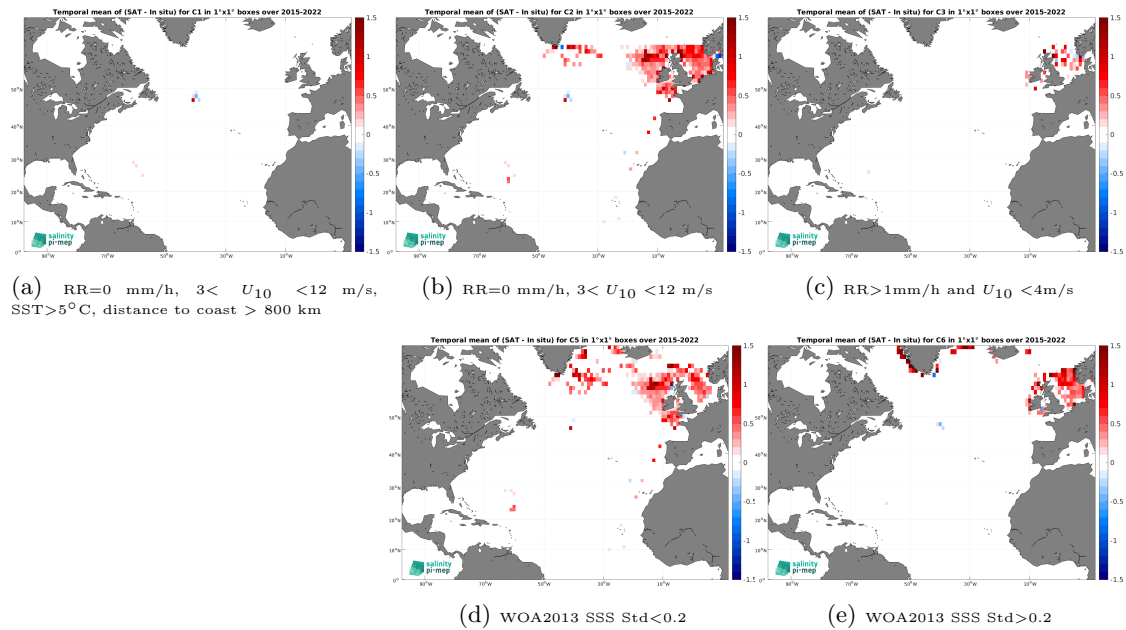
Figure 12: Temporal mean gridded over spatial boxes of size 1^\circ \times 1^\circ of \Delta\text{SSS} (SMAP SSS L3 v5 - Monthly (RSS) - ICES) for 5 different subdatasets corresponding to:RR=0 mm/h, 3 < U_{10} < 12 m/s, SST >5^\circ\text{C} , distance to coast > 800 km (a), RR=0 mm/h, 3 < U_{10} < 12 m/s (b), RR >1 mm/h and U_{10} < 4 m/s (c), WOA2013 SSS Std <0.2 (d), WOA2013 SSS Std >0.2 (e).
