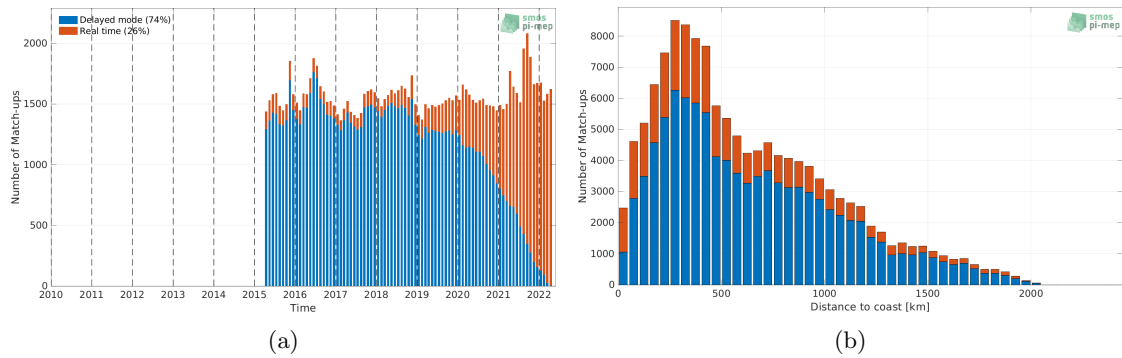
Figure 1: Number of match-ups between Argo and SMAP SSS L3 v5 - Monthly (RSS) SSS as a function of time (a) and as function of the distance to coast (b) over the North Atlantic Ocean Pi-MEP region and for the full satellite product period.
