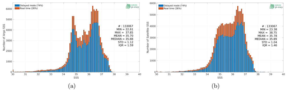
Figure 2: Histograms of SSS from Argo (a) and SMAP SSS L3 v5 - Monthly (RSS) (b) considering all match-up pairs per bins of 0.1 over the North Atlantic Ocean Pi-MEP region and for the full satellite product period.
