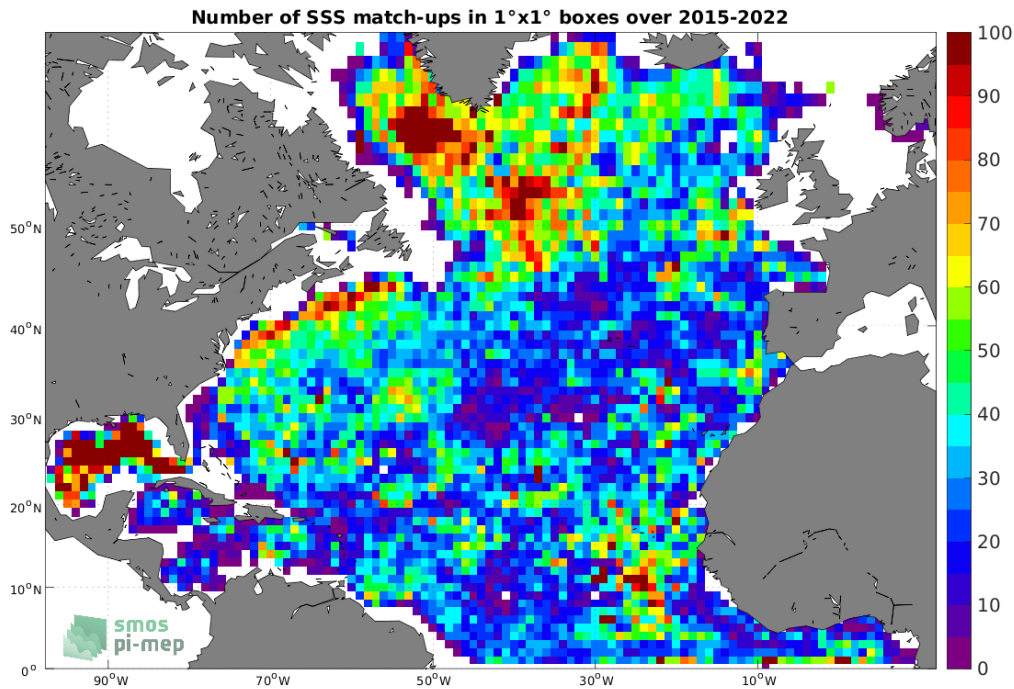
Figure 4: Number of SSS match-ups between Argo SSS and the SMAP SSS L3 v5 - Monthly (RSS) SSS product for the North Atlantic Ocean Pi-MEP region over 1^\circ \times 1^\circ boxes and for the full satellite product period.
