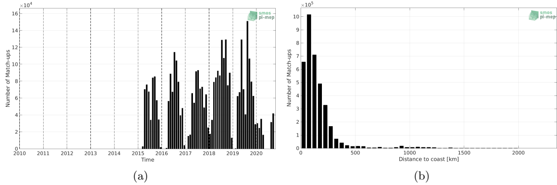
Figure 1: Number of match-ups between TSG (SAMOS) and SMAP SSS L3 v4 - 8-Day running (RSS) SSS as a function of time (a) and as function of the distance to the coast (b) over the North Atlantic Ocean Pi-MEP region and for the full satellite product period.
