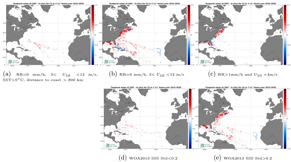
Figure 12: Temporal mean gridded over spatial boxes of size 1^\circ \times 1^\circ of \Delta\text{SSS} (SMAP SSS L3 v4 - 8-Day running (RSS) - TSG (SAMOS)) for 5 different subdatasets corresponding to:RR=0 mm/h, 3 < U_{10} < 12 m/s, SST > 5^\circ\text{C} , distance to coast > 800 km (a), RR=0 mm/h, 3 < U_{10} < 12 m/s (b), RR > 1 mm/h and U_{10} < 4 m/s (c), WOA2013 SSS Std < 0.2 (d), WOA2013 SSS Std > 0.2 (e).
