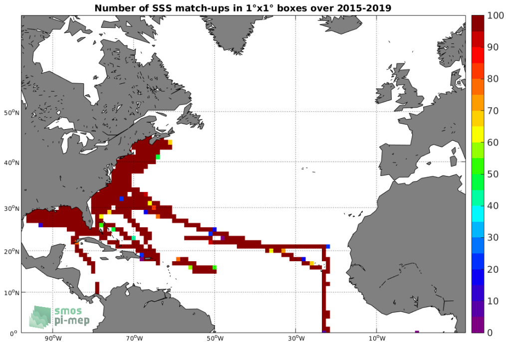
Figure 4: Number of SSS match-ups between TSG-SAMOS SSS and the SMAP-L3-RSS-V4-8DAY-RUNNING SSS product for the North Atlantic Ocean Pi-MEP region over 1^\circ \times 1^\circ boxes and for the full satellite product period.
