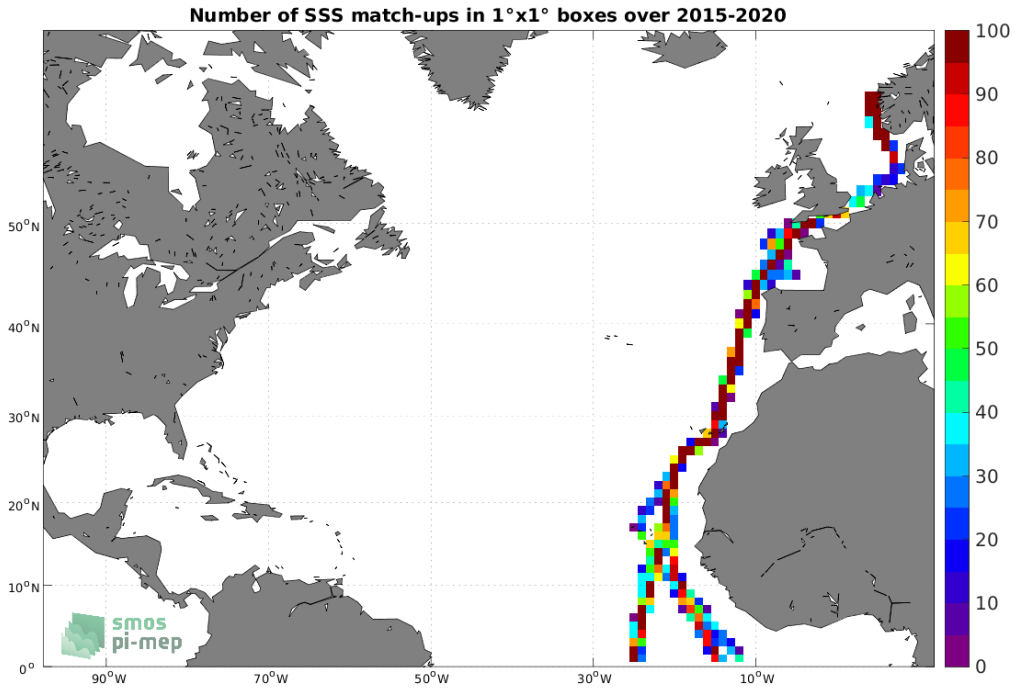
Figure 4: Number of SSS match-ups between TSG (Polarstern) SSS and the SMAP SSS L3 v4 - 8-Day running (RSS) SSS product for the North Atlantic Ocean Pi-MEP region over 1^\circ \times 1^\circ boxes and for the full satellite product period.
