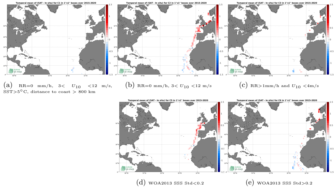
Figure 12: Temporal mean gridded over spatial boxes of size 1^\circ \times 1^\circ of \Delta SSS (SMAP SSS L3 v4 - 8-Day running (RSS) - TSG (Polarstern)) for 5 different subdatasets corresponding to:RR=0 mm/h, 3 < U_{10} < 12 m/s, SST >5^\circ\text{C} , distance to coast > 800 km (a), RR=0 mm/h, 3 < U_{10} < 12 m/s (b), RR >1 mm/h and U_{10} < 4 m/s (c), WOA2013 SSS Std <0.2 (d), WOA2013 SSS Std >0.2 (e).
