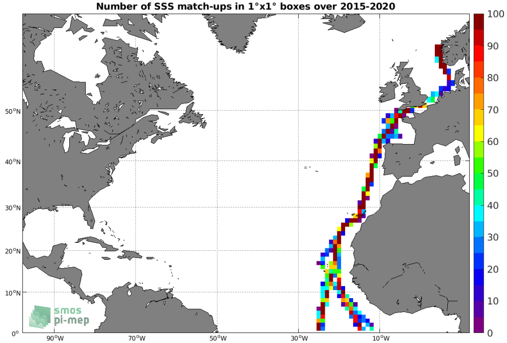
Figure 4: Number of SSS match-ups between TSG (Polarstern) SSS and the SMAP SSS L3 v4 - 8-Day running (RSS) SSS product for the North Atlantic Ocean Pi-MEP region over 1°x1° boxes and for the full satellite product period.
