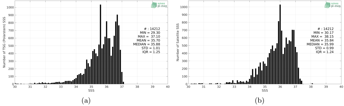
Figure 2: Histograms of SSS from TSG (Polarstern) (a) and SMAP SSS L3 v4 - 8-Day running (RSS) (b) considering all match-up pairs per bins of 0.1 over the North Atlantic Ocean Pi-MEP region and for the full satellite product period.
