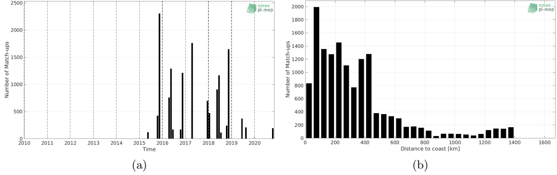
Figure 1: Number of match-ups between TSG (Polarstern) and SMAP SSS L3 v4 - 8-Day running (RSS) SSS as a function of time (a) and as function of the distance to coast (b) over the North Atlantic Ocean Pi-MEP region and for the full satellite product period.
