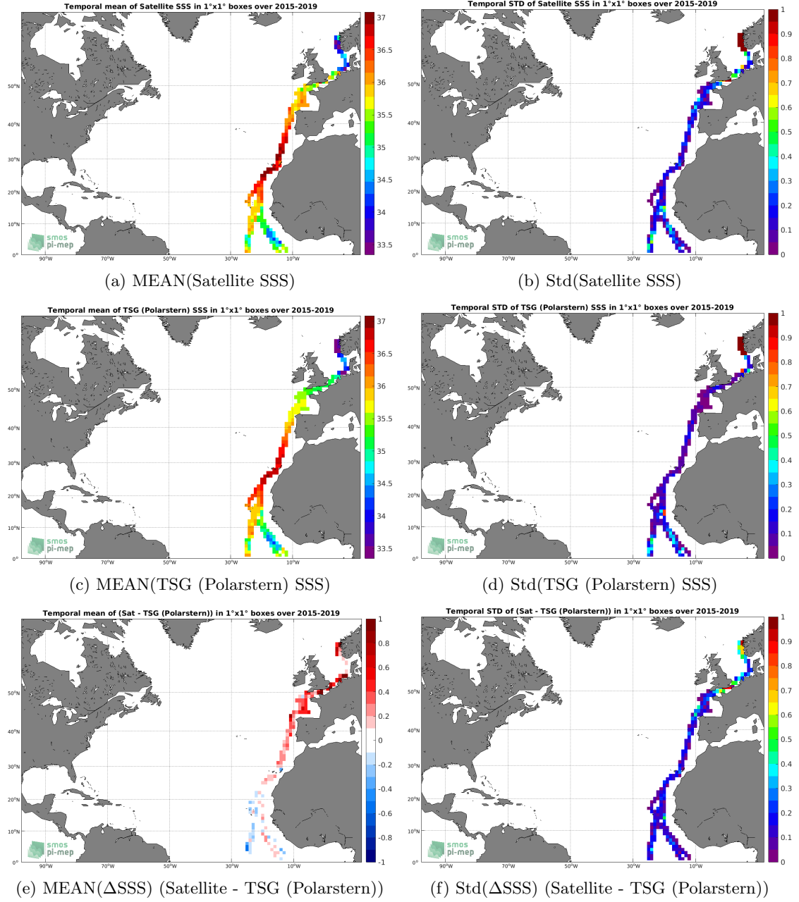
Figure 6: Temporal mean (left) and Std (right) of SSS from SMAP SSS L3 v4 - 8-Day running (RSS) (top), TSG (Polarstern) (middle), and of \Delta SSS (Satellite - TSG (Polarstern)). Only match-up pairs are used to generate these maps.
