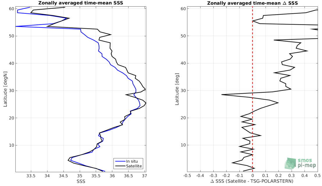
Figure 8: Left panel: Zonal mean SSS from SMAP-L3-RSS-V4-8DAY-RUNNING satellite product (black) and from TSG-POLARSTERN (blue). Right panel: Zonal mean of \Delta SSS (Satellite - TSG-POLARSTERN) for all the collected Pi-MEP match-up pairs estimated over the full satellite product period.
