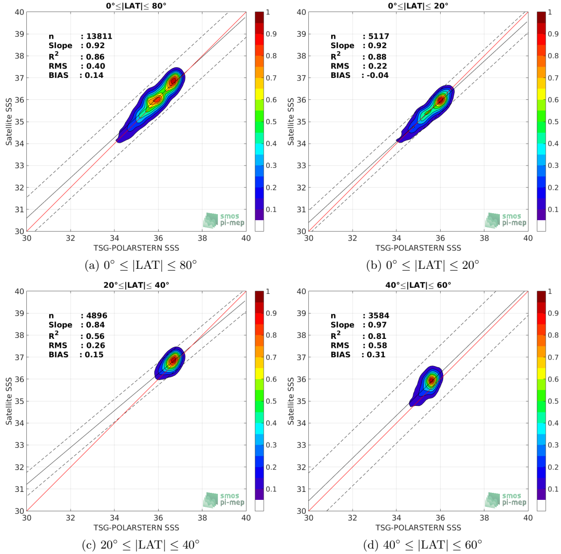
Figure 9: Contour maps of the concentration of SMAP-L3-RSS-V4-8DAY-RUNNING SSS (y-axis) versus TSG-POLARSTERN SSS (x-axis) at match-up pairs for different latitude bands. For each plot, the red line shows x=y . The black thin and dashed lines indicate a linear fit through the data cloud and the \pm 95\% confidence levels, respectively. The number match-up pairs n , the slope and R^2 coefficient of the linear fit, the root mean square (RMS) and the mean bias between satellite and in situ data are indicated for each latitude band in each plots.
