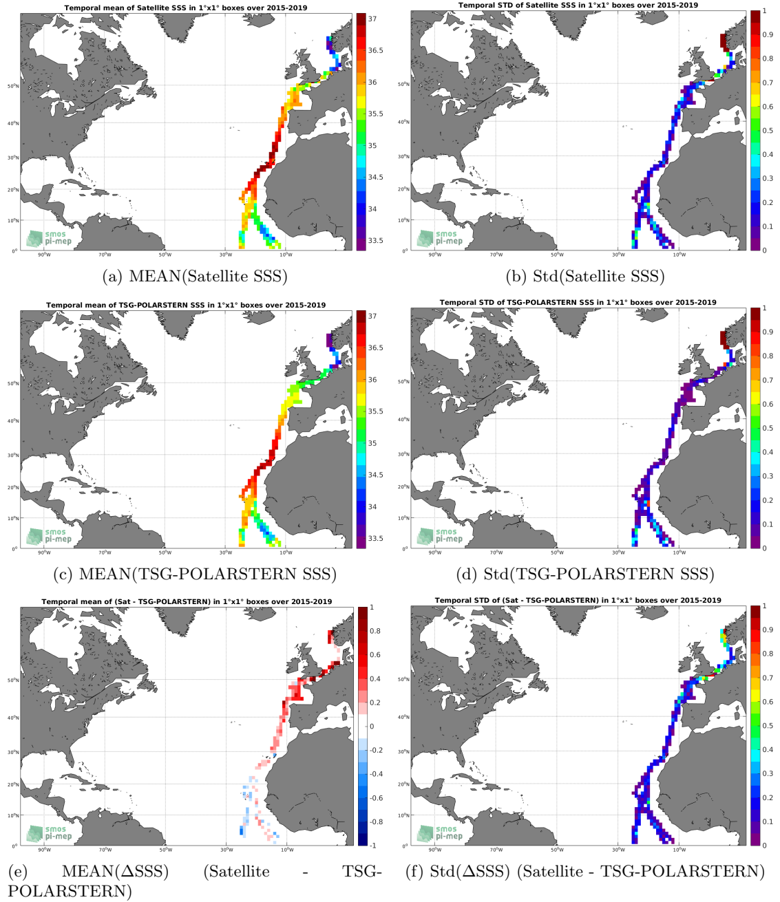
Figure 6: Temporal mean (left) and Std (right) of SSS from SMAP-L3-RSS-V4-8DAY-RUNNING (top), TSG-POLARSTERN (middle), and of \Delta SSS (Satellite - TSG-POLARSTERN). Only match-up pairs are used to generate these maps.
