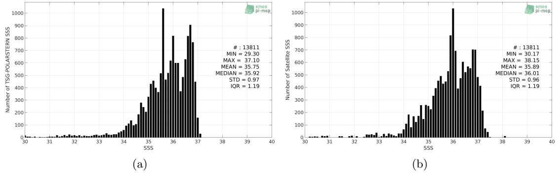
Figure 2: Histograms of SSS from TSG-POLARSTERN (a) and SMAP-L3-RSS-V4-8DAY-RUNNING (b) considering all match-up pairs per bins of 0.1 over the North Atlantic Ocean Pi-MEP region and for the full satellite product period.
