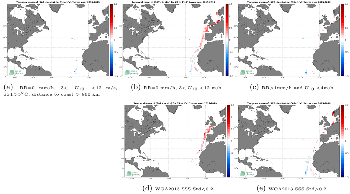
Figure 12: Temporal mean gridded over spatial boxes of size 1^\circ \times 1^\circ of \Delta SSS (SMAP-L3-RSS-V4-8DAY-RUNNING - TSG-POLARSTERN) for 5 different subdatasets corresponding to: RR=0 mm/h, 3 < U_{10} < 12 m/s, SST > 5^\circ\text{C} , distance to coast > 800 km (a), RR=0 mm/h, 3 < U_{10} < 12 m/s (b), RR > 1 mm/h and U_{10} < 4 m/s (c), WOA2013 SSS Std < 0.2 (d), WOA2013 SSS Std > 0.2 (e).
