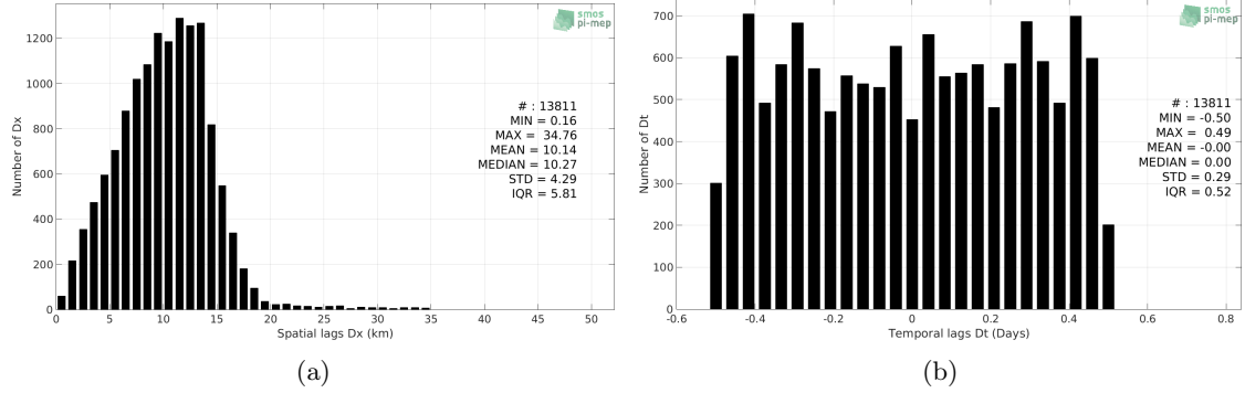
Figure 5: Histograms of the spatial (a) and temporal (b) lags between the time of the TSG-POLARSTERN measurements and the date of the corresponding SMAP-L3-RSS-V4-8DAY-RUNNING SSS product.
