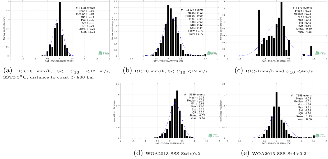
Figure 13: Normalized histogram of \Delta SSS (SMAP-L3-RSS-V4-8DAY-RUNNING - TSG-POLARSTERN) for 5 different subdatasets corresponding to: RR=0 mm/h, 3 < U_{10} < 12 m/s, SST > 5°C, distance to coast > 800 km (a), RR=0 mm/h, 3 < U_{10} < 12 m/s (b), RR > 1 mm/h and U_{10} < 4 m/s (c), WOA2013 SSS Std < 0.2 (d), WOA2013 SSS Std > 0.2 (e).
