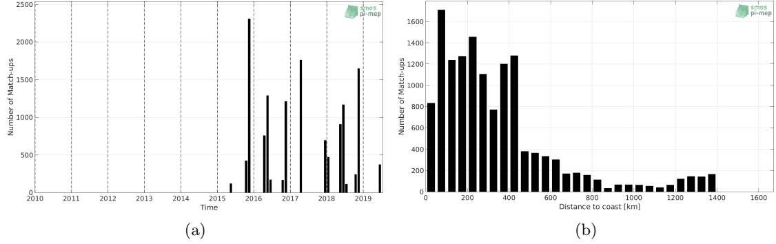
Figure 1: Number of match-ups between TSG-POLARSTERN and SMAP-L3-RSS-V4-8DAY-RUNNING SSS as a function of time (a) and as function of the distance to coast (b) over the North Atlantic Ocean Pi-MEP region and for the full satellite product period.
