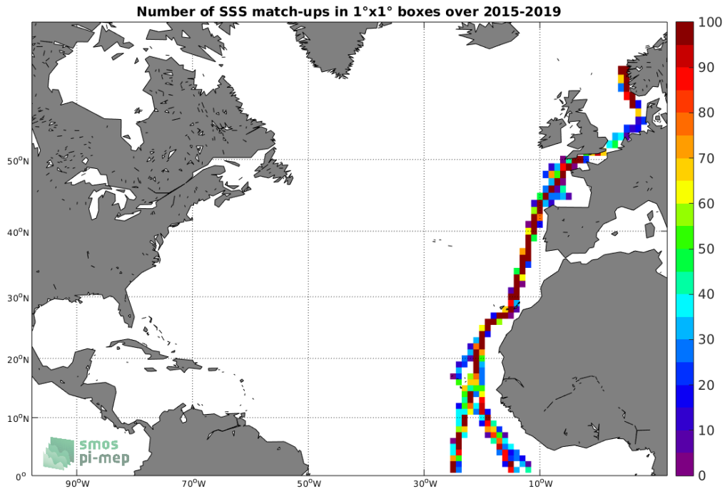
Figure 4: Number of SSS match-ups between TSG-POLARSTERN SSS and the SMAP-L3-RSS-V4-8DAY-RUNNING SSS product for the North Atlantic Ocean Pi-MEP region over 1^\circ \times 1^\circ boxes and for the full satellite product period.
