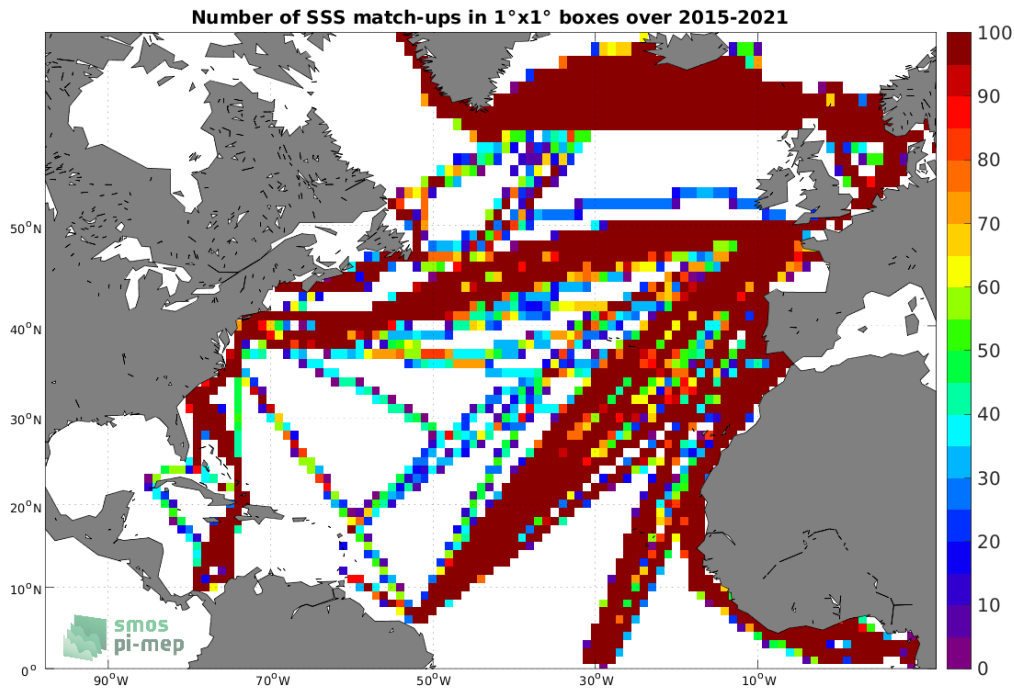
Figure 4: Number of SSS match-ups between TSG (LEGOS-DM) SSS and the SMAP SSS L3 v4 - 8-Day running (RSS) SSS product for the North Atlantic Ocean Pi-MEP region over 1^\circ \times 1^\circ boxes and for the full satellite product period.
