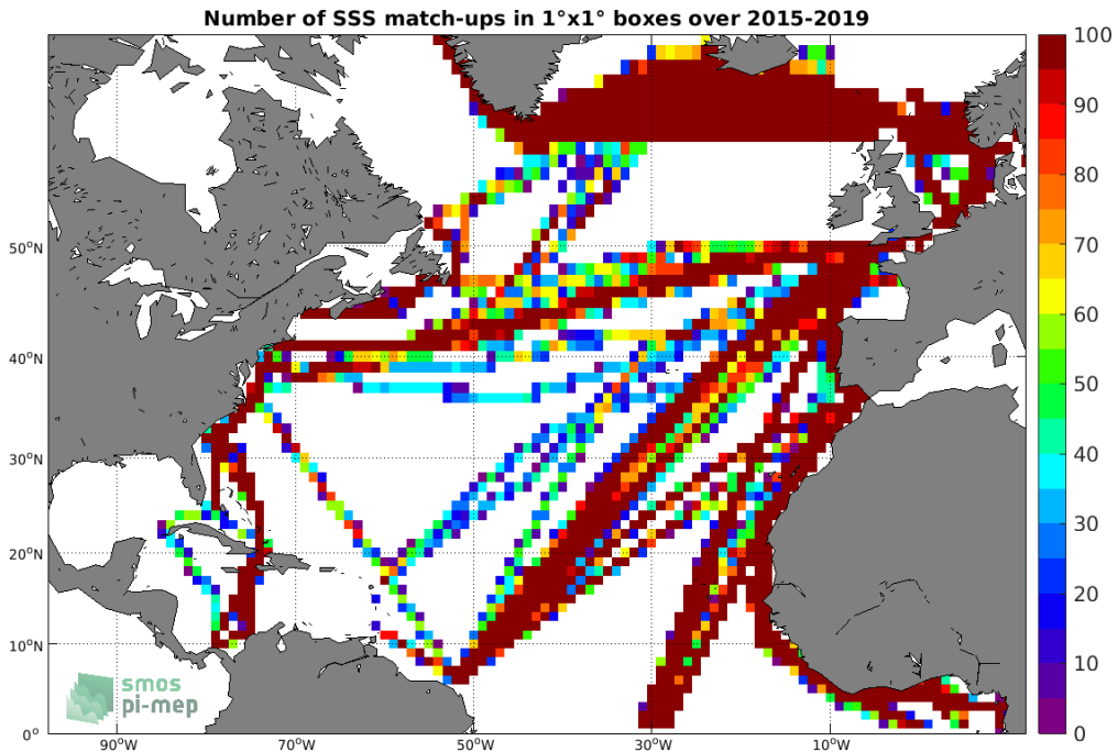
Figure 4: Number of SSS match-ups between TSG (LEGOS-DM) SSS and the SMAP SSS L3 v4 - 8-Day running (RSS) SSS product for the North Atlantic Ocean Pi-MEP region over 1°x1° boxes and for the full satellite product period.
