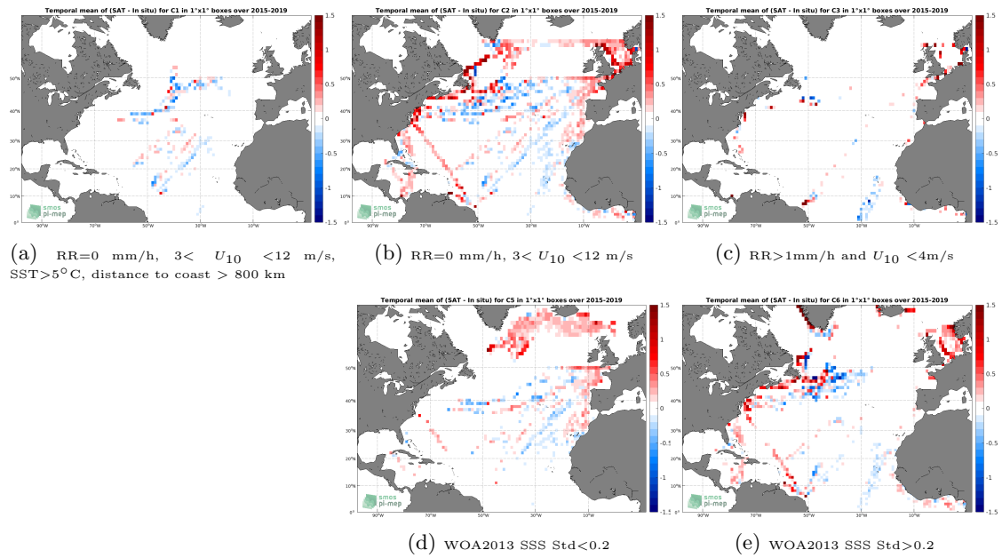
Figure 12: Temporal mean gridded over spatial boxes of size 1^\circ \times 1^\circ of \Delta\text{SSS} (SMAP SSS L3 v4 - 8-Day running (RSS) - TSG (LEGOS-DM)) for 5 different subdatasets corresponding to:RR=0 mm/h, 3 < U_{10} < 12 m/s, SST > 5^\circ\text{C} , distance to coast > 800 km (a), RR=0 mm/h, 3 < U_{10} < 12 m/s (b), RR > 1 mm/h and U_{10} < 4 m/s (c), WOA2013 SSS Std < 0.2 (d), WOA2013 SSS Std > 0.2 (e).
