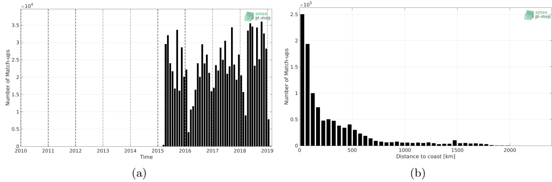
Figure 1: Number of match-ups between TSG (LEGOS-DM) and SMAP SSS L3 v4 - 8-Day running (RSS) SSS as a function of time (a) and as function of the distance to coast (b) over the North Atlantic Ocean Pi-MEP region and for the full satellite product period.
