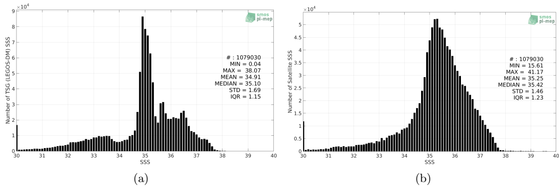
Figure 2: Histograms of SSS from TSG (LEGOS-DM) (a) and SMAP SSS L3 v4 - 8-Day running (RSS) (b) considering all match-up pairs per bins of 0.1 over the North Atlantic Ocean Pi-MEP region and for the full satellite product period.
