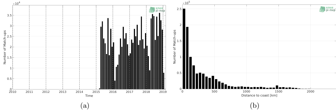
Figure 1: Number of match-ups between TSG-LEGOS-DM and SMAP-L3-RSS-V4-8DAY-RUNNING SSS as a function of time (a) and as function of the distance to coast (b) over the North Atlantic Ocean Pi-MEP region and for the full satellite product period.
