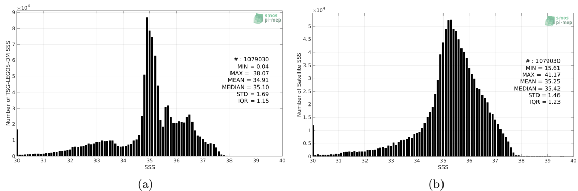
Figure 2: Histograms of SSS from TSG-LEGOS-DM (a) and SMAP-L3-RSS-V4-8DAY-RUNNING (b) considering all match-up pairs per bins of 0.1 over the North Atlantic Ocean Pi-MEP region and for the full satellite product period.
