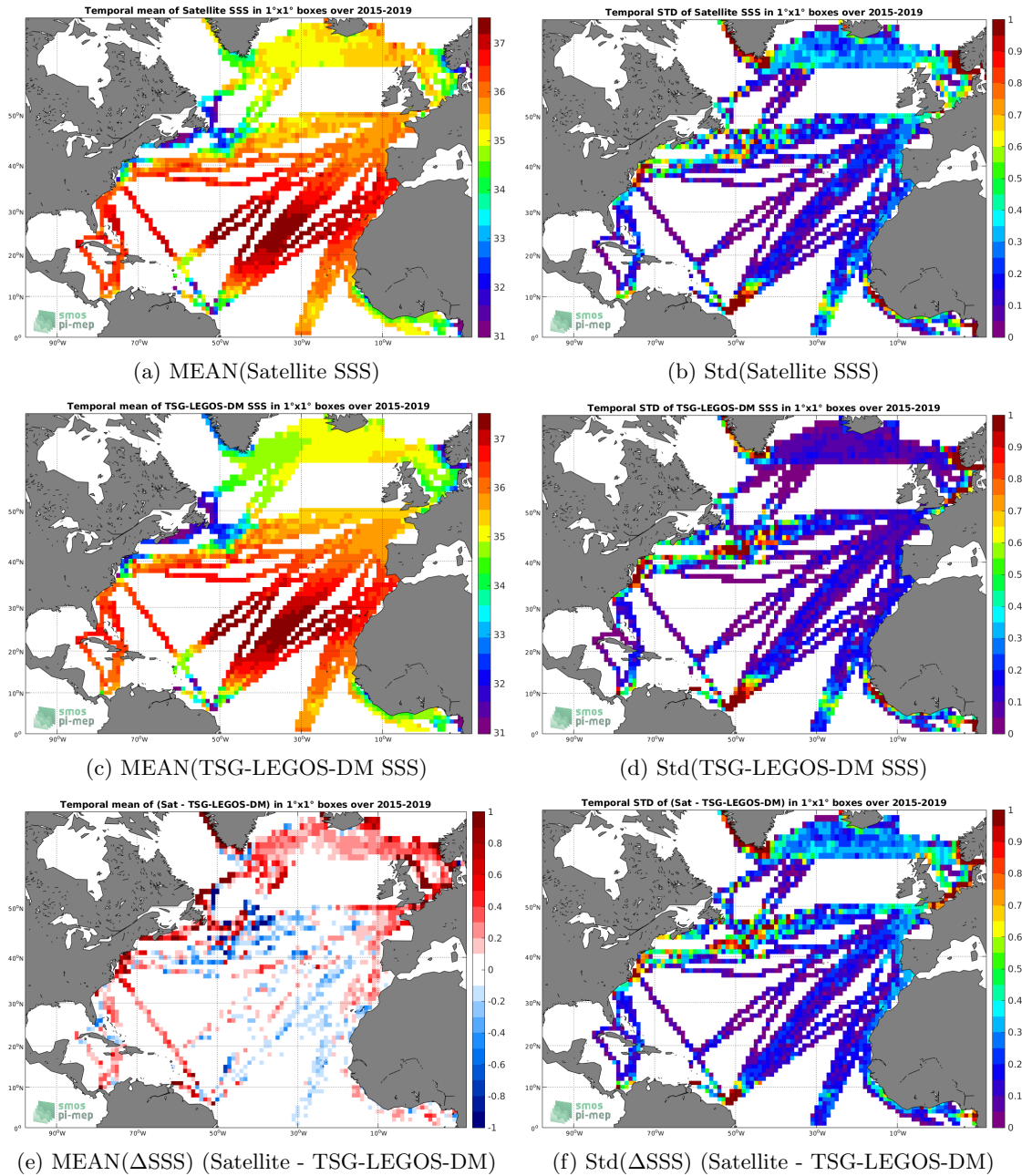
Figure 6: Temporal mean (left) and Std (right) of SSS from SMAP-L3-RSS-V4-8DAY-RUNNING (top), TSG-LEGOS-DM (middle), and of \Delta SSS (Satellite - TSG-LEGOS-DM). Only match-up pairs are used to generate these maps.
