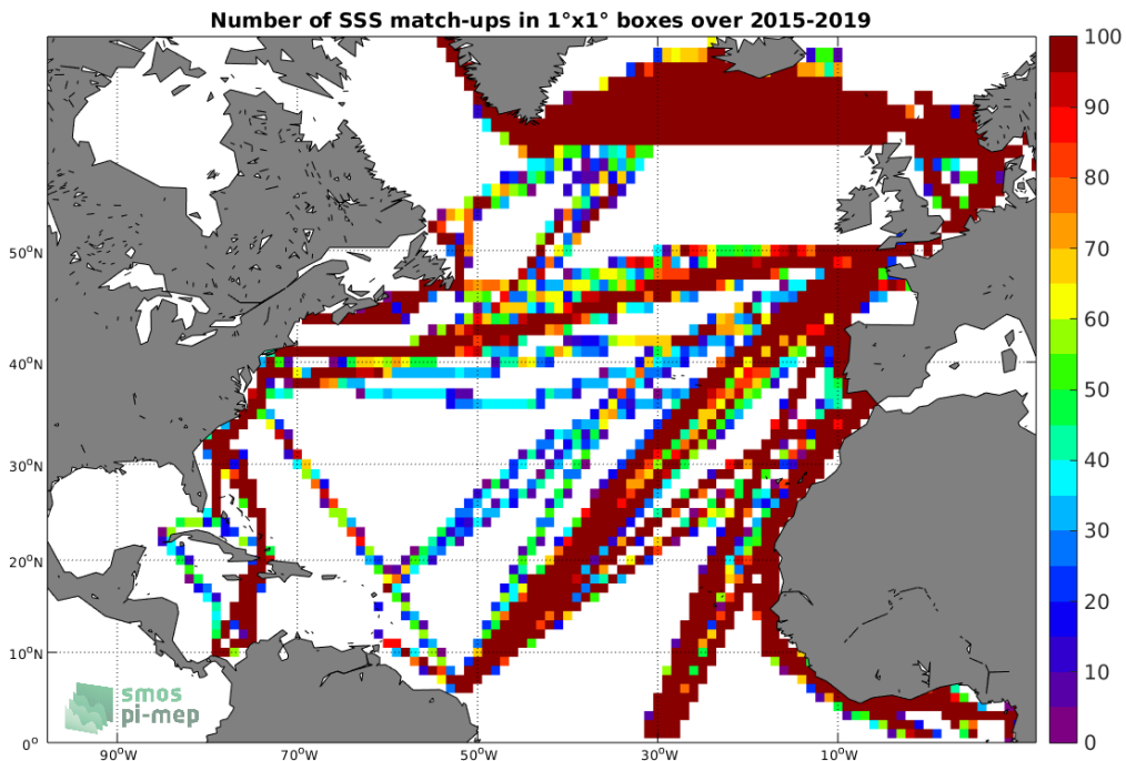
Figure 4: Number of SSS match-ups between TSG-LEGOS-DM SSS and the SMAP-L3-RSS-V4-8DAY-RUNNING SSS product for the North Atlantic Ocean Pi-MEP region over 1^\circ \times 1^\circ boxes and for the full satellite product period.
