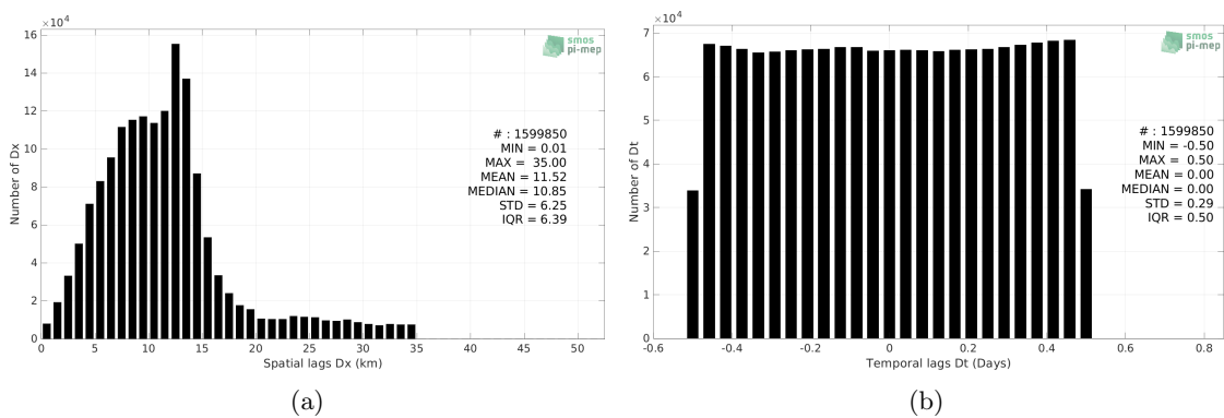
Figure 5: Histograms of the spatial (a) and temporal (b) lags between the location/time of the TSG (GOSUD-Research-vessel) measurement and the date of the corresponding SMAP SSS L3 v4 - 8-Day running (RSS) SSS pixel.
