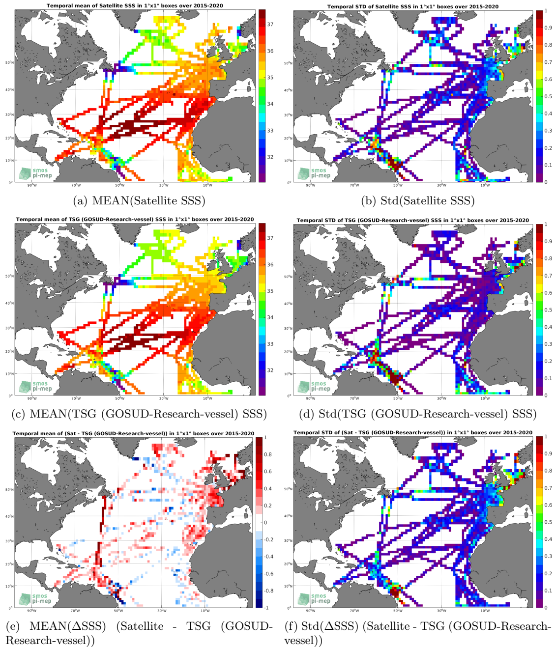
Figure 6: Temporal mean (left) and Std (right) of SSS from SMAP SSS L3 v4 - 8-Day running (RSS) (top), TSG (GOSUD-Research-vessel) (middle), and of \Delta SSS (Satellite - TSG (GOSUD-Research-vessel)). Only match-up pairs are used to generate these maps.
