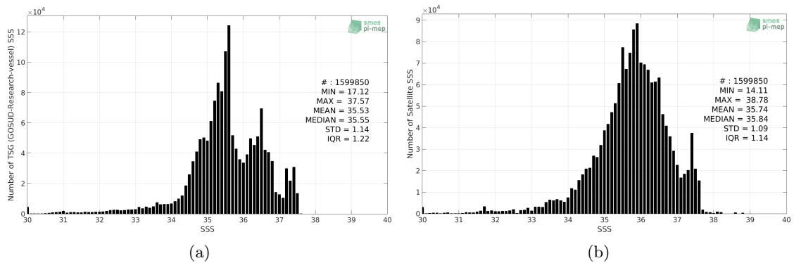
Figure 2: Histograms of SSS from TSG (GOSUD-Research-vessel) (a) and SMAP SSS L3 v4 - 8-Day running (RSS) (b) considering all match-up pairs per bins of 0.1 over the North Atlantic Ocean Pi-MEP region and for the full satellite product period.
