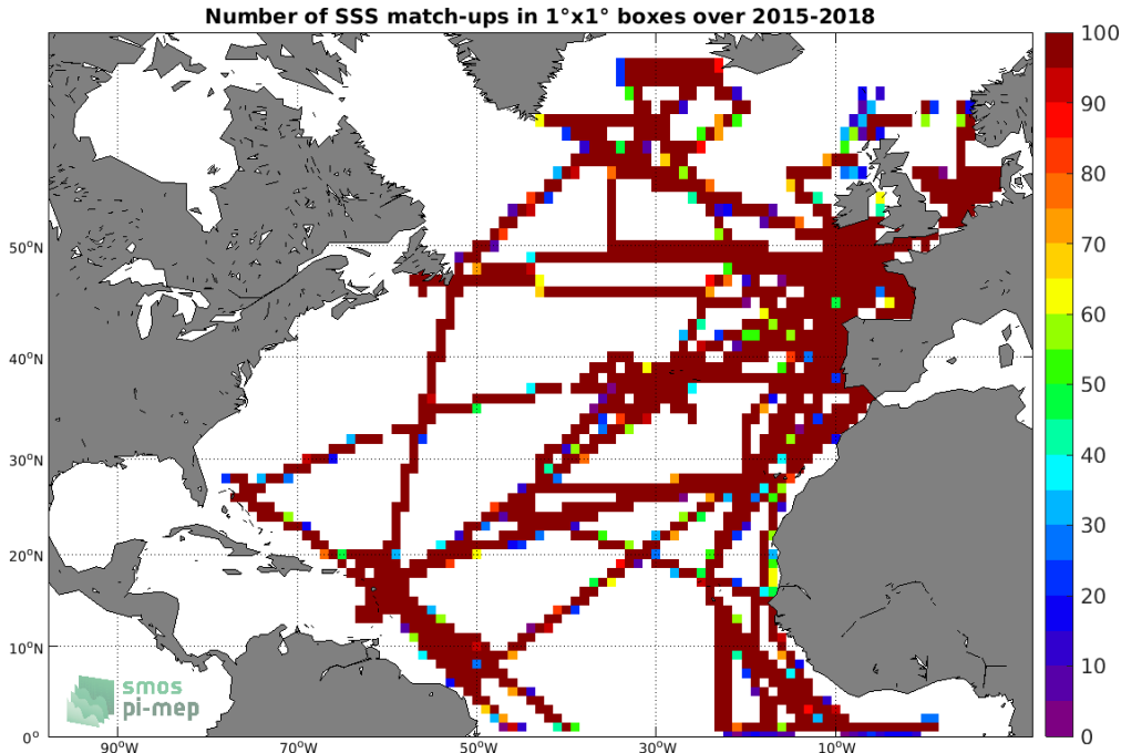
Figure 4: Number of SSS match-ups between TSG (GOSUD-Research-vessel) SSS and the SMAP SSS L3 v4 - 8-Day running (RSS) SSS product for the North Atlantic Ocean Pi-MEP region over 1°x1° boxes and for the full satellite product period.
