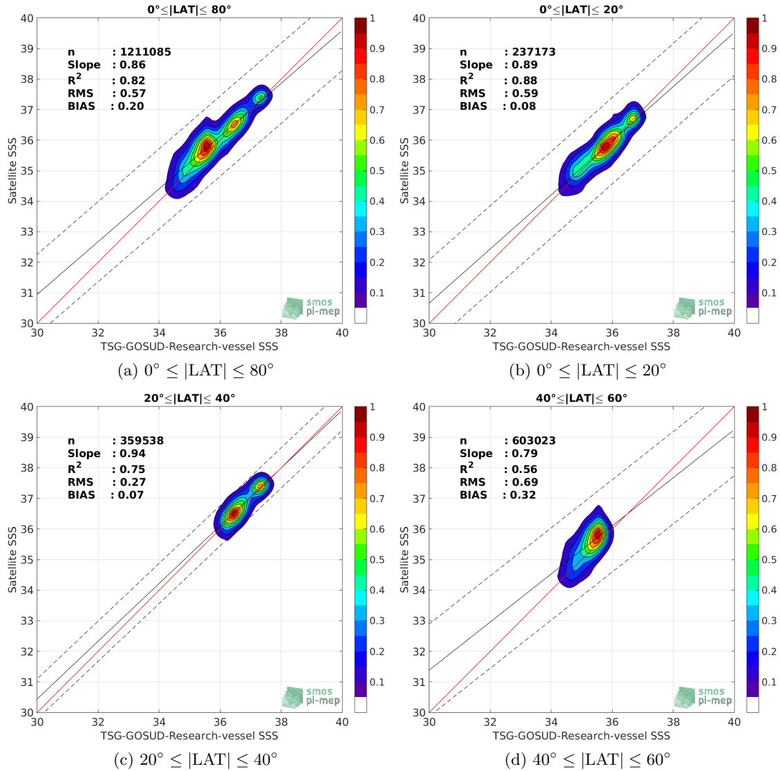
Figure 9: Contour maps of the concentration of SMAP-L3-RSS-V4-8DAY-RUNNING SSS ( y -axis) versus TSG-GOSUD-Research-vessel SSS ( x -axis) at match-up pairs for different latitude bands. For each plot, the red line shows x=y . The black thin and dashed lines indicate a linear fit through the data cloud and the \pm 95\% confidence levels, respectively. The number match-up pairs n , the slope and R^2 coefficient of the linear fit, the root mean square (RMS) and the mean bias between satellite and in situ data are indicated for each latitude band in each plots.
