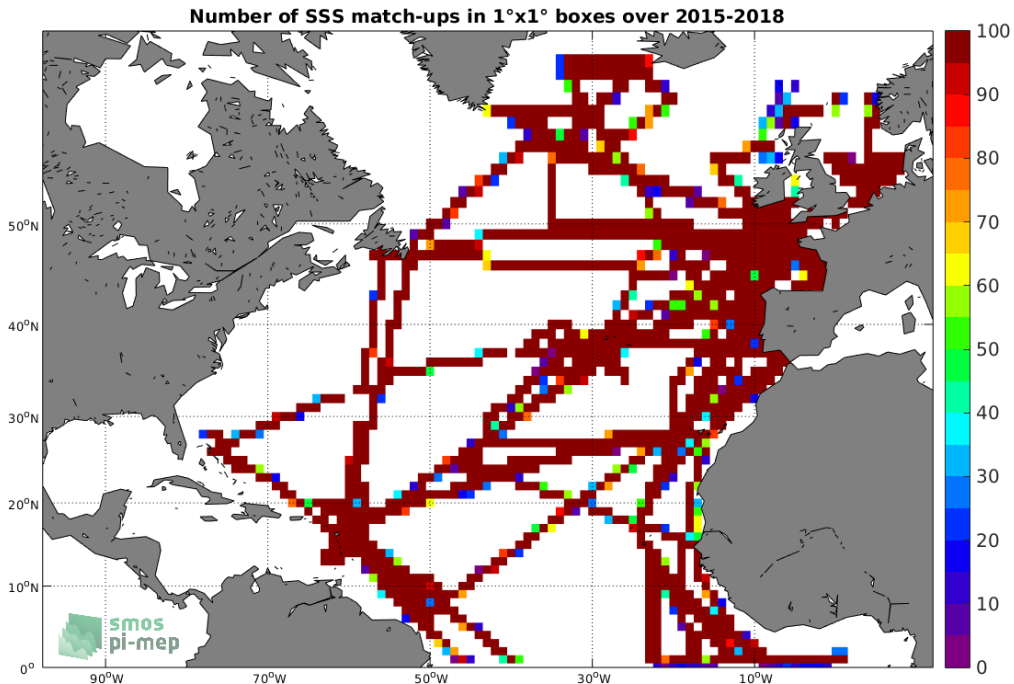
Figure 4: Number of SSS match-ups between TSG-GOSUD-Research-vessel SSS and the SMAP-L3-RSS-V4-8DAY-RUNNING SSS product for the North Atlantic Ocean Pi-MEP region over 1^\circ \times 1^\circ boxes and for the full satellite product period.
