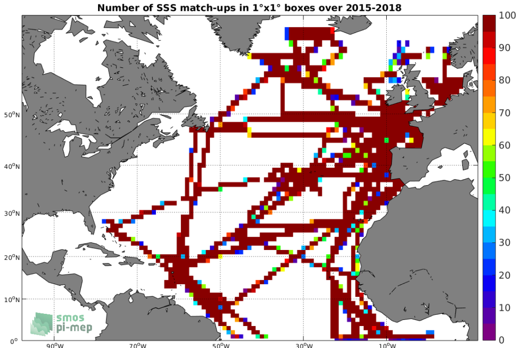
Figure 4: Number of SSS match-ups between TSG-GOSUD-Research-vessel SSS and the SMAP-L3-RSS-V4-8DAY-RUNNING SSS product for the North Atlantic Ocean Pi-MEP region over 1°x1° boxes and for the full satellite product period.
