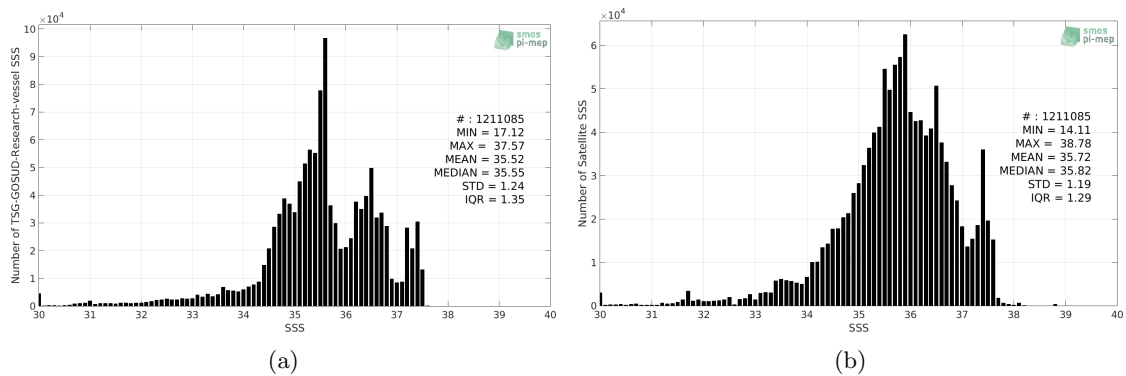
Figure 2: Histograms of SSS from TSG-GOSUD-Research-vessel (a) and SMAP-L3-RSS-V4-8DAY-RUNNING (b) considering all match-up pairs per bins of 0.1 over the North Atlantic Ocean Pi-MEP region and for the full satellite product period.
