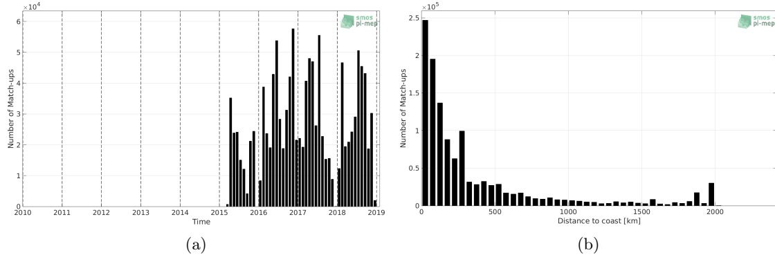
Figure 1: Number of match-ups between TSG-GOSUD-Research-vessel and SMAP-L3-RSS-V4-8DAY-RUNNING SSS as a function of time (a) and as function of the distance to coast (b) over the North Atlantic Ocean Pi-MEP region and for the full satellite product period.
