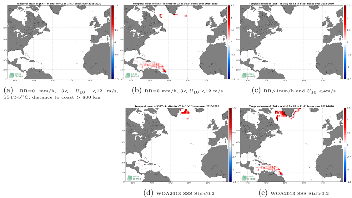
Figure 11: Temporal mean gridded over spatial boxes of size 1^\circ \times 1^\circ of \Delta\text{SSS} (SMAP SSS L3 v4 - 8-Day running (RSS) - Surface drifters) for 5 different subdatasets corresponding to:RR=0 mm/h, 3 < U_{10} < 12 m/s, SST > 5^\circ\text{C} , distance to coast > 800 km (a), RR=0 mm/h, 3 < U_{10} < 12 m/s (b), RR > 1 mm/h and U_{10} < 4 m/s (c), WOA2013 SSS Std < 0.2 (d), WOA2013 SSS Std > 0.2 (e).
