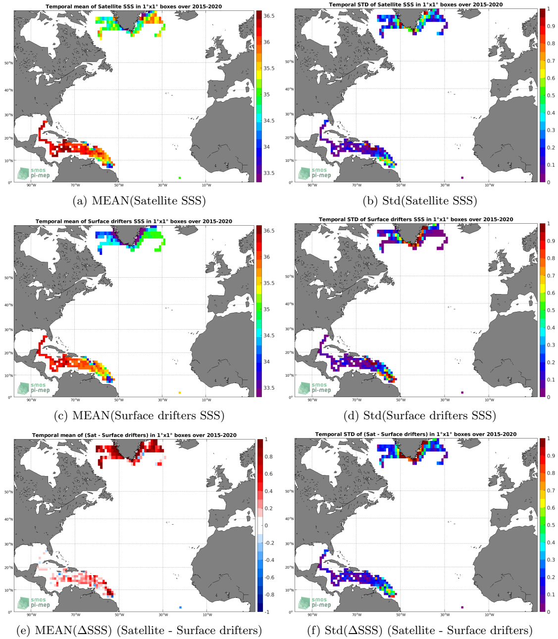
Figure 5: Temporal mean (left) and Std (right) of SSS from SMAP SSS L3 v4 - 8-Day running (RSS) (top), Surface drifters (middle), and of \Delta SSS (Satellite - Surface drifters). Only match-up pairs are used to generate these maps.
