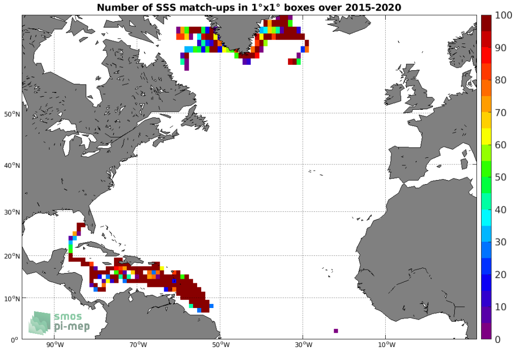
Figure 3: Number of SSS match-ups between Surface drifters SSS and the SMAP SSS L3 v4 - 8-Day running (RSS) SSS product for the North Atlantic Ocean Pi-MEP region over 1^\circ \times 1^\circ boxes and for the full satellite product period.
