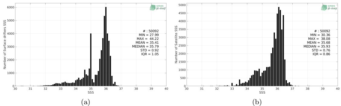
Figure 2: Histograms of SSS from Surface drifters (a) and SMAP SSS L3 v4 - 8-Day running (RSS) (b) considering all match-up pairs per bins of 0.1 over the North Atlantic Ocean Pi-MEP region and for the full satellite product period.
