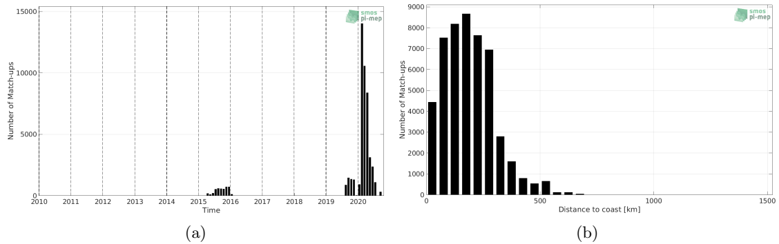
Figure 1: Number of match-ups between Surface drifters and SMAP SSS L3 v4 - 8-Day running (RSS) SSS as a function of time (a) and as function of the distance to coast (b) over the North Atlantic Ocean Pi-MEP region and for the full satellite product period.
