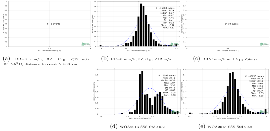
Figure 12: Normalized histogram of \Delta SSS (SMAP SSS L3 v4 - 8-Day running (RSS) - Surface drifters) for 5 different subdatasets corresponding to: RR=0 mm/h, 3 < U_{10} < 12 m/s, SST > 5°C, distance to coast > 800 km (a), RR=0 mm/h, 3 < U_{10} < 12 m/s (b), RR > 1mm/h and U_{10} < 4 m/s (c), WOA2013 SSS Std < 0.2 (d), WOA2013 SSS Std > 0.2 (e).
