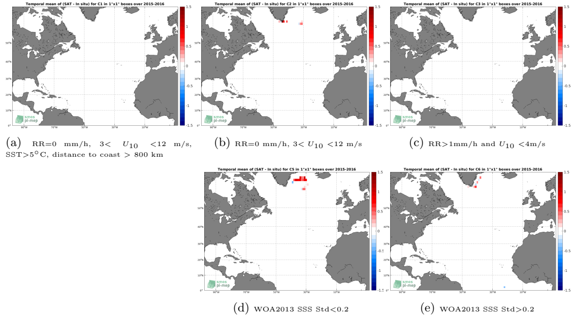
Figure 11: Temporal mean gridded over spatial boxes of size 1^{\circ}\times 1^{\circ} of \Delta\text{SSS} (SMAP SSS L3 v4 - 8-Day running (RSS) - Surface drifters) for 5 different subdatasets corresponding to:RR=0 mm/h, 3 < U_{10} < 12 m/s, SST >5^{\circ}\text{C} , distance to coast > 800 km (a), RR=0 mm/h, 3 < U_{10} < 12 m/s (b), RR >1 mm/h and U_{10} < 4 m/s (c), WOA2013 SSS Std <0.2 (d), WOA2013 SSS Std >0.2 (e).
