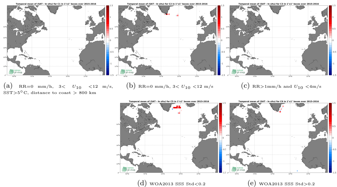
Figure 11: Temporal mean gridded over spatial boxes of size 1^{\circ}\times 1^{\circ} of \Delta\text{SSS} (SMAP-L3-RSS-V4-8DAY-RUNNING - Surface drifters) for 5 different subdatasets corresponding to:RR=0 mm/h, 3 < U_{10} < 12 m/s, SST >5^{\circ}\text{C} , distance to coast > 800 km (a), RR=0 mm/h, 3 < U_{10} < 12 m/s (b), RR >1 mm/h and U_{10} < 4 m/s (c), WOA2013 SSS Std <0.2 (d), WOA2013 SSS Std >0.2 (e).
