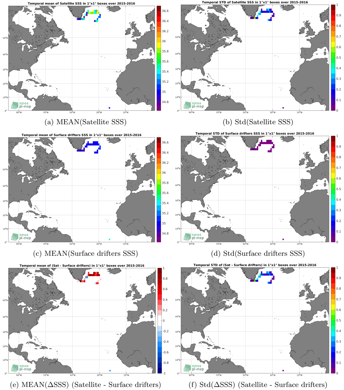
Figure 5: Temporal mean (left) and Std (right) of SSS from SMAP-L3-RSS-V4-8DAY-RUNNING (top), Surface drifters (middle), and of \Delta SSS (Satellite - Surface drifters). Only match-up pairs are used to generate these maps.
