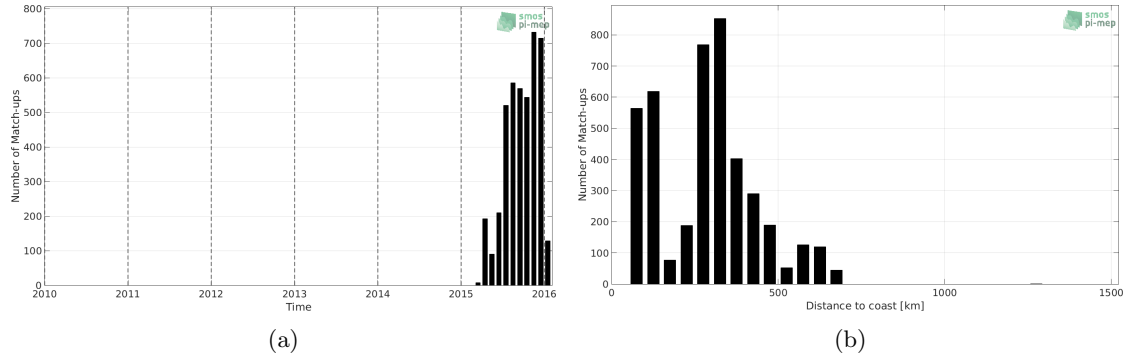
Figure 1: Number of match-ups between Surface drifters and SMAP-L3-RSS-V4-8DAY-RUNNING SSS as a function of time (a) and as function of the distance to coast (b) over the North Atlantic Ocean Pi-MEP region and for the full satellite product period.
