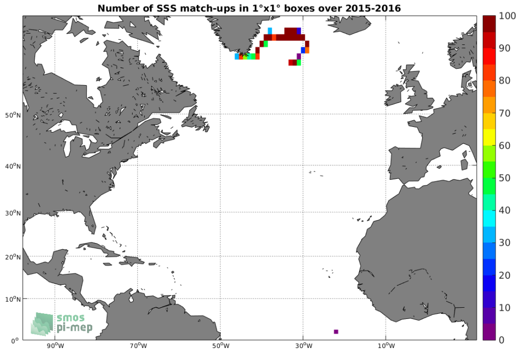
Figure 3: Number of SSS match-ups between Surface drifters SSS and the SMAP-L3-RSS-V4-8DAY-RUNNING SSS product for the North Atlantic Ocean Pi-MEP region over 1^\circ \times 1^\circ boxes and for the full satellite product period.
