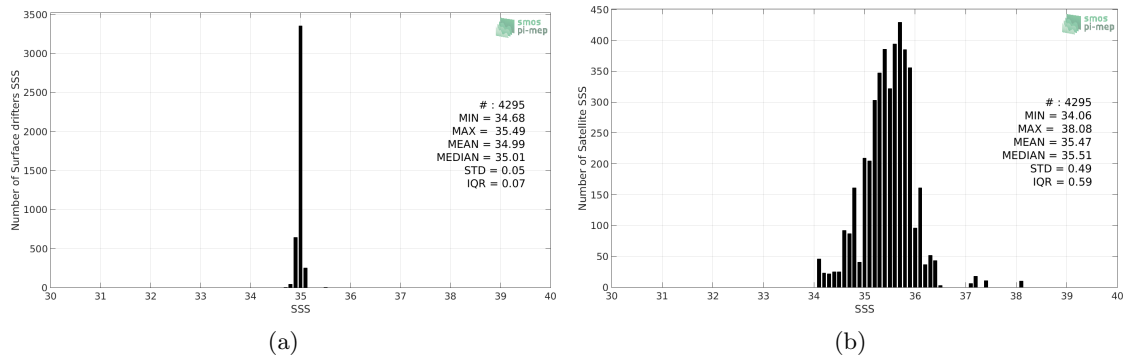
Figure 2: Histograms of SSS from Surface drifters (a) and SMAP-L3-RSS-V4-8DAY-RUNNING (b) considering all match-up pairs per bins of 0.1 over the North Atlantic Ocean Pi-MEP region and for the full satellite product period.
