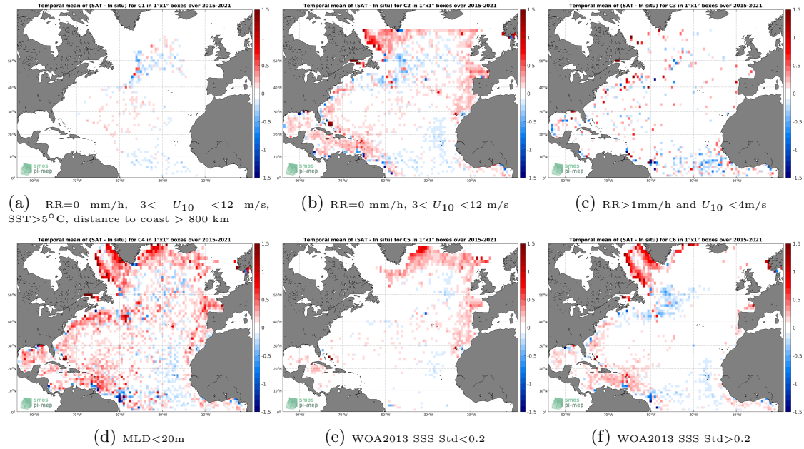
Figure 12: Temporal mean gridded over spatial boxes of size 1^\circ \times 1^\circ of \Delta SSS (SMAP SSS L3 v4 - 8-Day running (RSS) - Argo) for 6 different subdatasets corresponding to: RR=0 mm/h, 3 < U_{10} < 12 m/s, SST > 5^\circ C , distance to coast > 800 km (a), RR=0 mm/h, 3 < U_{10} < 12 m/s (b), RR > 1 mm/h and U_{10} < 4 m/s (c), MLD < 20 m (d), WOA2013 SSS Std < 0.2 (e), WOA2013 SSS Std > 0.2 (f).
