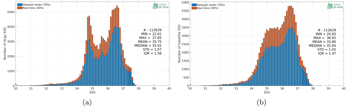
Figure 2: Histograms of SSS from Argo (a) and SMAP SSS L3 v4 - 8-Day running (RSS) (b) considering all match-up pairs per bins of 0.1 over the North Atlantic Ocean Pi-MEP region and for the full satellite product period.
