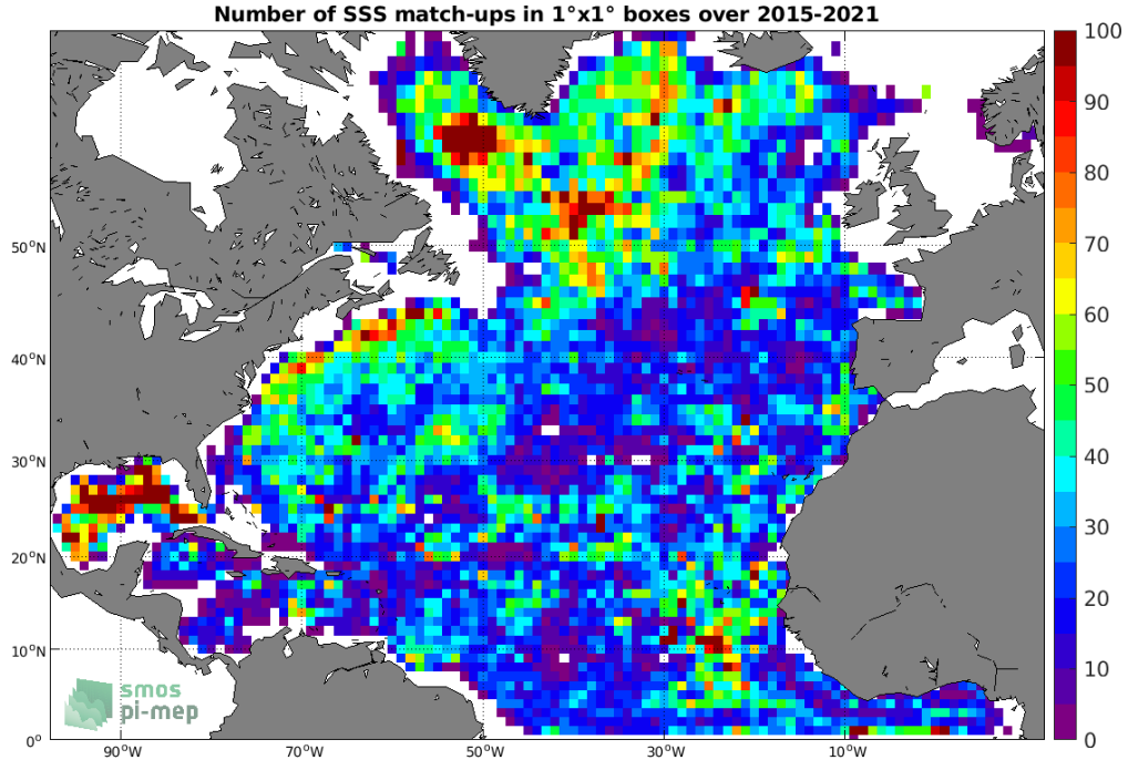
Figure 4: Number of SSS match-ups between Argo SSS and the SMAP SSS L3 v4 - 8-Day running (RSS) SSS product for the North Atlantic Ocean Pi-MEP region over 1°x1° boxes and for the full satellite product period.
