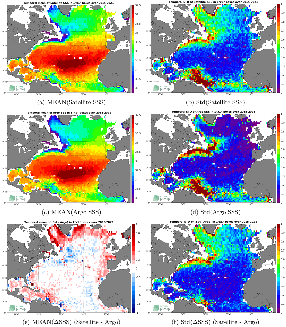
Figure 6: Temporal mean (left) and Std (right) of SSS from SMAP SSS L3 v4 - 8-Day running (RSS) (top), Argo (middle), and of \Delta SSS (Satellite - Argo). Only match-up pairs are used to generate these maps.
