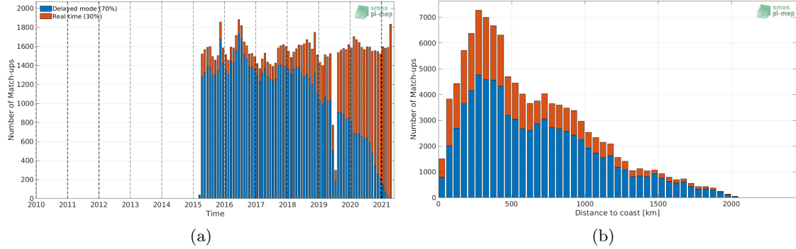
Figure 1: Number of match-ups between Argo and SMAP SSS L3 v4 - 8-Day running (RSS) SSS as a function of time (a) and as function of the distance to coast (b) over the North Atlantic Ocean Pi-MEP region and for the full satellite product period.
