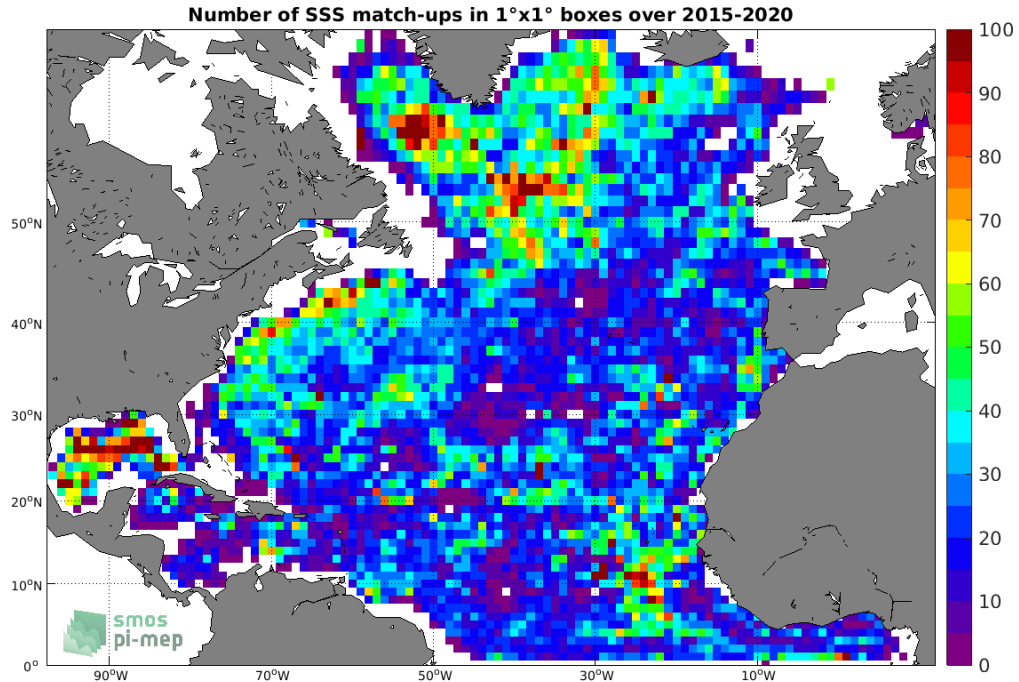
Figure 4: Number of SSS match-ups between Argo SSS and the SMAP SSS L3 v4 - 8-Day running (RSS) SSS product for the North Atlantic Ocean Pi-MEP region over 1^\circ \times 1^\circ boxes and for the full satellite product period.
