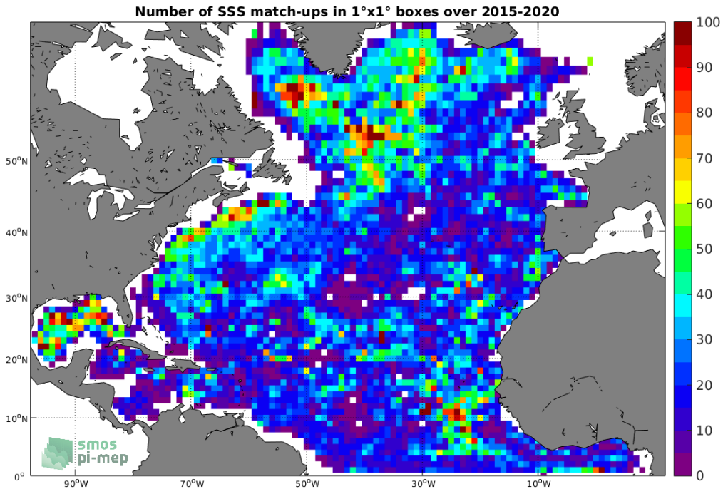
Figure 4: Number of SSS match-ups between Argo SSS and the SMAP-L3-RSS-V4-8DAY-RUNNING SSS product for the North Atlantic Ocean Pi-MEP region over 1^\circ \times 1^\circ boxes and for the full satellite product period.
