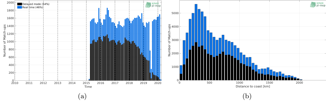
Figure 1: Number of match-ups between Argo and SMAP-L3-RSS-V4-8DAY-RUNNING SSS as a function of time (a) and as function of the distance to coast (b) over the North Atlantic Ocean Pi-MEP region and for the full satellite product period.
