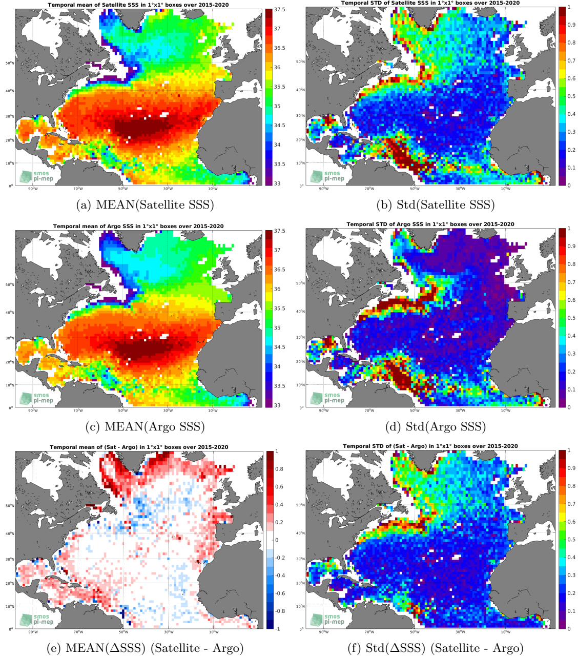
Figure 6: Temporal mean (left) and Std (right) of SSS from SMAP-L3-RSS-V4-8DAY-RUNNING (top), Argo (middle), and of \Delta SSS (Satellite - Argo). Only match-up pairs are used to generate these maps.
