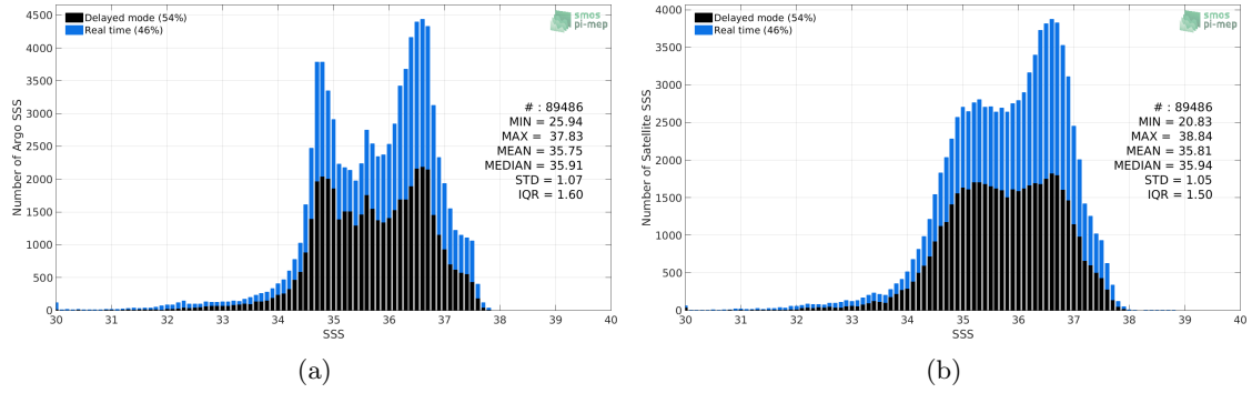
Figure 2: Histograms of SSS from Argo (a) and SMAP-L3-RSS-V4-8DAY-RUNNING (b) considering all match-up pairs per bins of 0.1 over the North Atlantic Ocean Pi-MEP region and for the full satellite product period.
