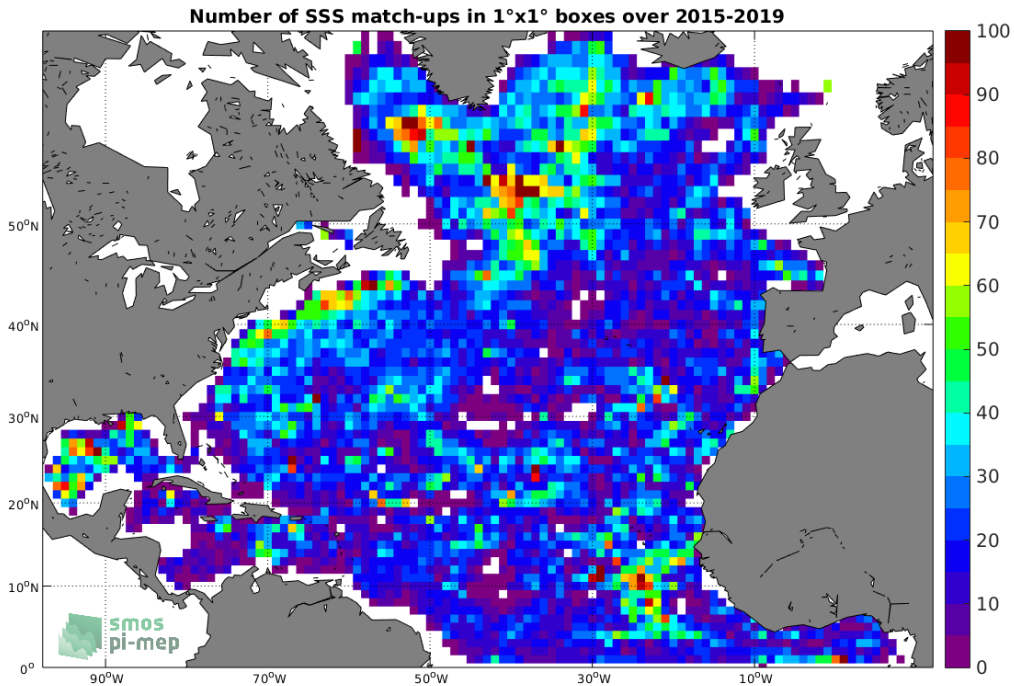
Figure 4: Number of SSS match-ups between Argo SSS and the SMAP-L3-RSS-V4-8DAY-RUNNING SSS product for the North Atlantic Ocean Pi-MEP region over 1°x1° boxes and for the full satellite product period.
