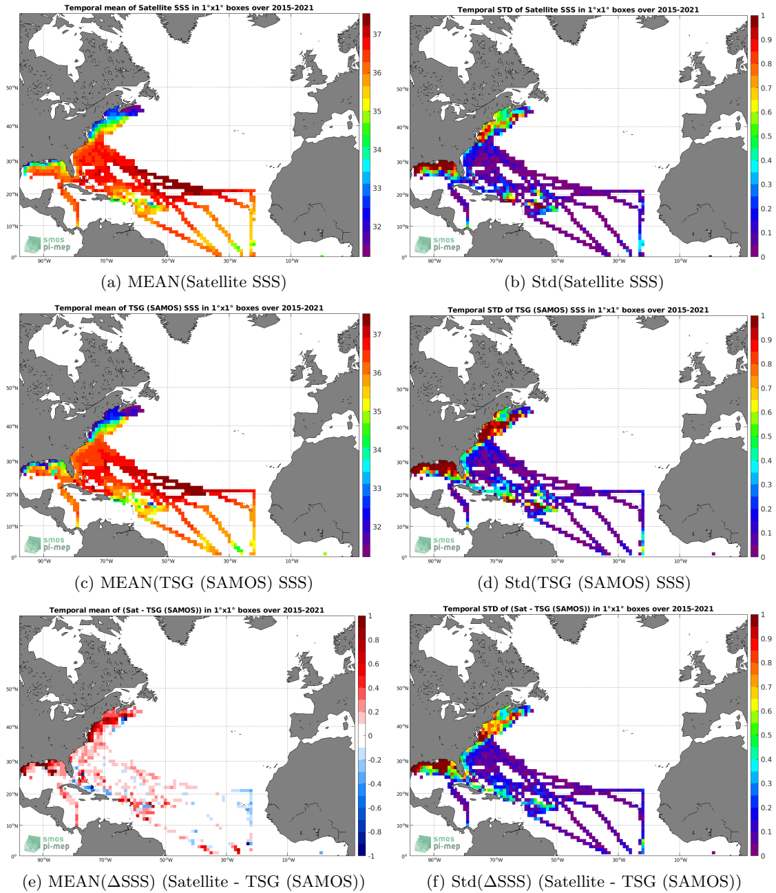
Figure 6: Temporal mean (left) and Std (right) of SSS from SMAP SSS L3 v4 - Monthly (RSS) (top), TSG (SAMOS) (middle), and of \Delta SSS (Satellite - TSG (SAMOS)). Only match-up pairs are used to generate these maps.
