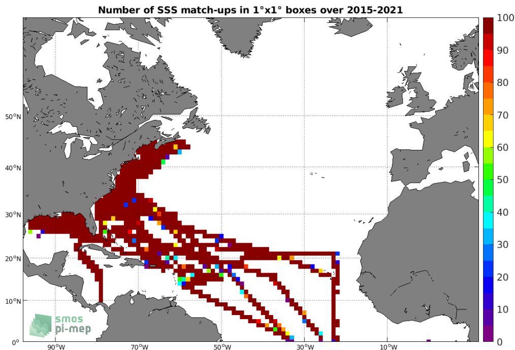
Figure 4: Number of SSS match-ups between TSG (SAMOS) SSS and the SMAP SSS L3 v4 - Monthly (RSS) SSS product for the North Atlantic Ocean Pi-MEP region over 1^\circ \times 1^\circ boxes and for the full satellite product period.
