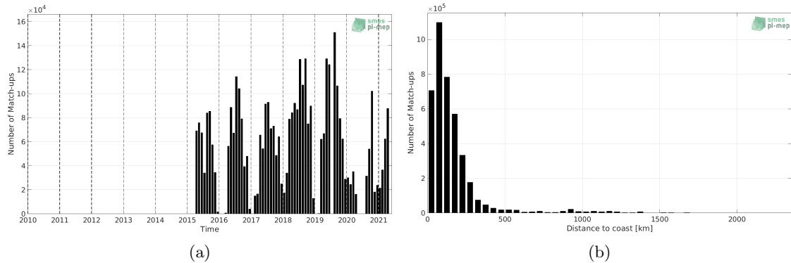
Figure 1: Number of match-ups between TSG (SAMOS) and SMAP SSS L3 v4 - Monthly (RSS) SSS as a function of time (a) and as function of the distance to coast (b) over the North Atlantic Ocean Pi-MEP region and for the full satellite product period.
