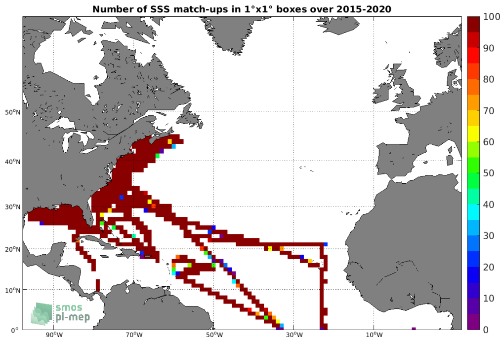
Figure 4: Number of SSS match-ups between TSG (SAMOS) SSS and the SMAP SSS L3 v4 - Monthly (RSS) SSS product for the North Atlantic Ocean Pi-MEP region over 1°x1° boxes and for the full satellite product period.
