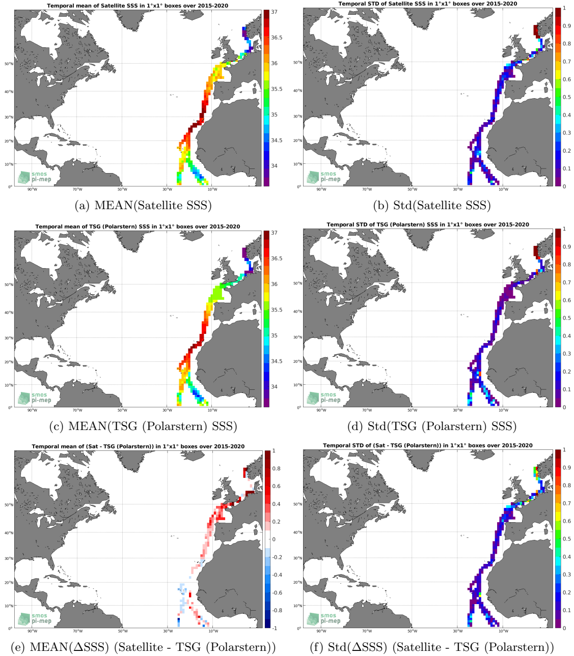
Figure 6: Temporal mean (left) and Std (right) of SSS from SMAP SSS L3 v4 - Monthly (RSS) (top), TSG (Polarstern) (middle), and of \Delta SSS (Satellite - TSG (Polarstern)). Only match-up pairs are used to generate these maps.
