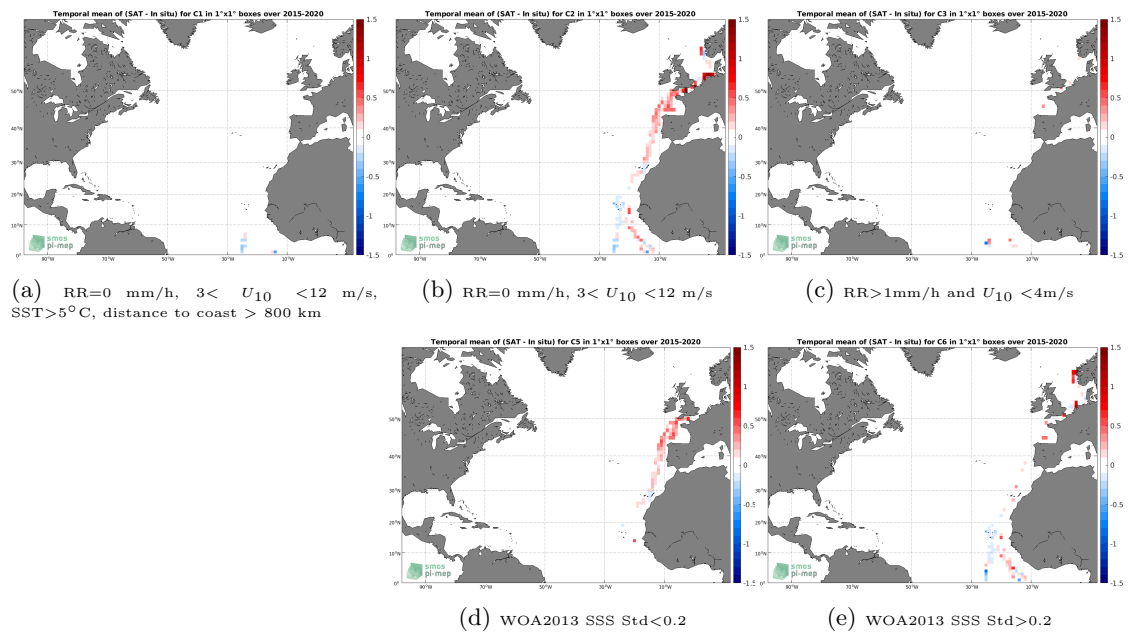
Figure 12: Temporal mean gridded over spatial boxes of size 1^\circ \times 1^\circ of \Delta SSS (SMAP SSS L3 v4 - Monthly (RSS) - TSG (Polarstern)) for 5 different subdatasets corresponding to:RR=0 mm/h, 3 < U_{10} < 12 m/s, SST >5^\circ\text{C} , distance to coast > 800 km (a), RR=0 mm/h, 3 < U_{10} < 12 m/s (b), RR >1 mm/h and U_{10} < 4 m/s (c), WOA2013 SSS Std <0.2 (d), WOA2013 SSS Std >0.2 (e).
