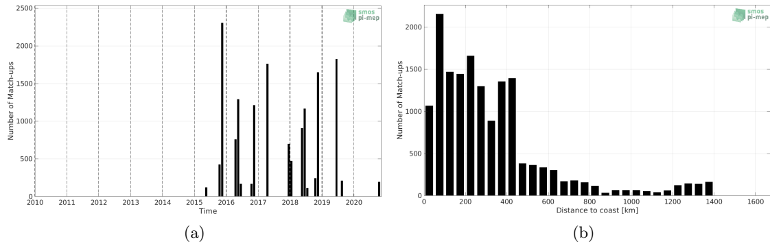
Figure 1: Number of match-ups between TSG (Polarstern) and SMAP SSS L3 v4 - Monthly (RSS) SSS as a function of time (a) and as function of the distance to coast (b) over the North Atlantic Ocean Pi-MEP region and for the full satellite product period.
