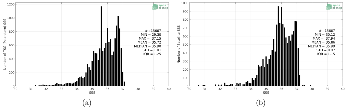
Figure 2: Histograms of SSS from TSG (Polarstern) (a) and SMAP SSS L3 v4 - Monthly (RSS) (b) considering all match-up pairs per bins of 0.1 over the North Atlantic Ocean Pi-MEP region and for the full satellite product period.
