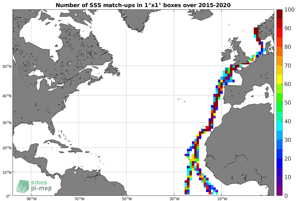
Figure 4: Number of SSS match-ups between TSG (Polarstern) SSS and the SMAP SSS L3 v4 - Monthly (RSS) SSS product for the North Atlantic Ocean Pi-MEP region over 1^\circ \times 1^\circ boxes and for the full satellite product period.
