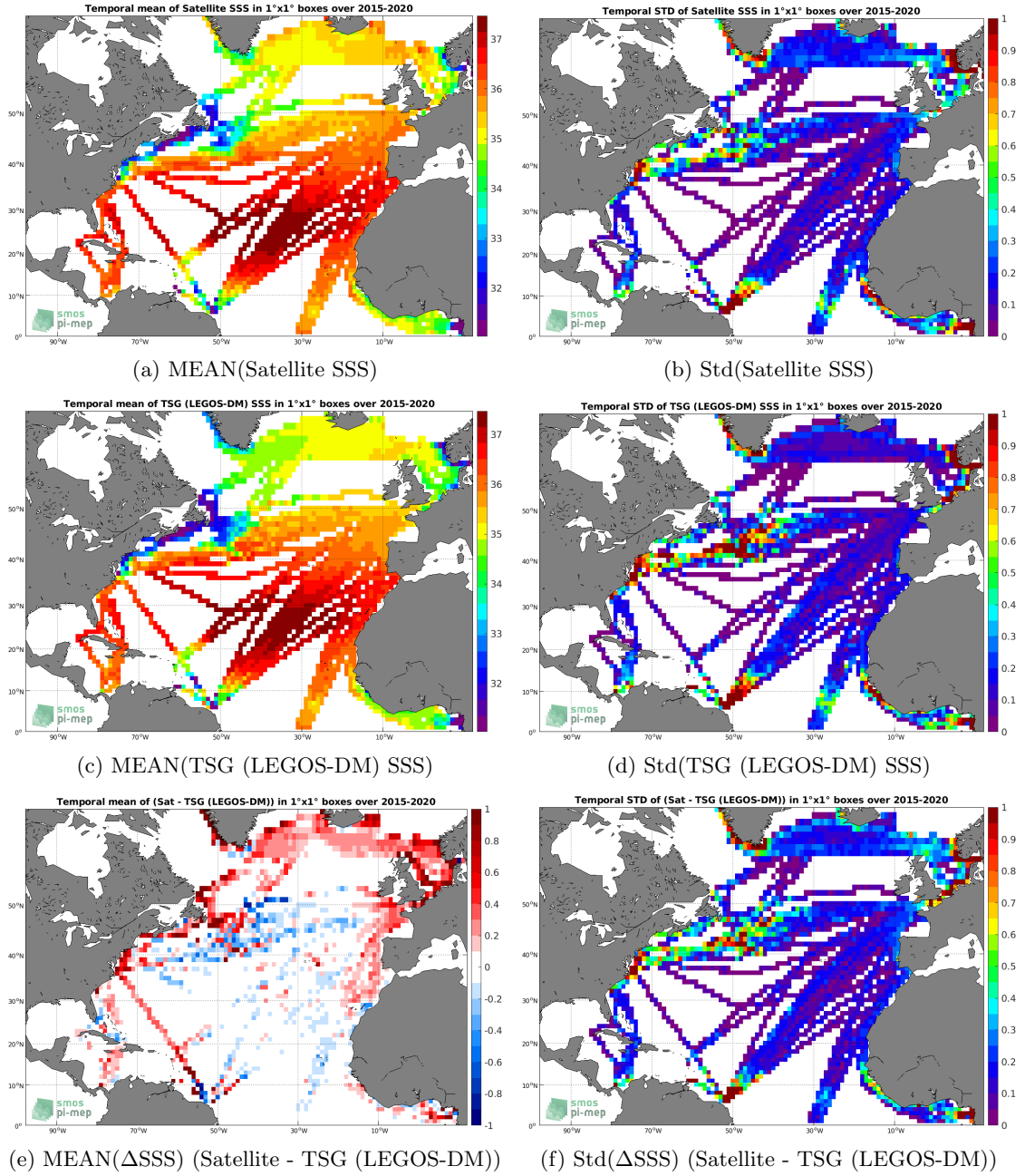
Figure 6: Temporal mean (left) and Std (right) of SSS from SMAP SSS L3 v4 - Monthly (RSS) (top), TSG (LEGOS-DM) (middle), and of \Delta SSS (Satellite - TSG (LEGOS-DM)). Only match-pairs are used to generate these maps.
