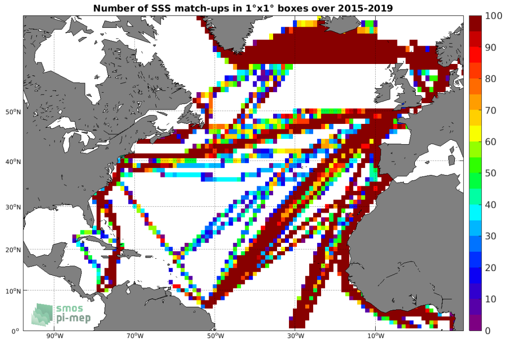
Figure 4: Number of SSS match-ups between TSG (LEGOS-DM) SSS and the SMAP SSS L3 v4 - Monthly (RSS) SSS product for the North Atlantic Ocean Pi-MEP region over 1^\circ \times 1^\circ boxes and for the full satellite product period.
