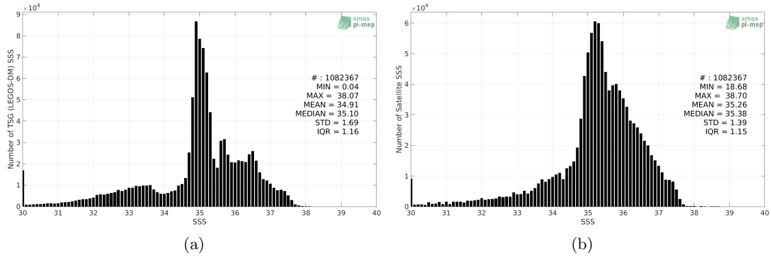
Figure 2: Histograms of SSS from TSG (LEGOS-DM) (a) and SMAP SSS L3 v4 - Monthly (RSS) (b) considering all match-up pairs per bins of 0.1 over the North Atlantic Ocean Pi-MEP region and for the full satellite product period.
