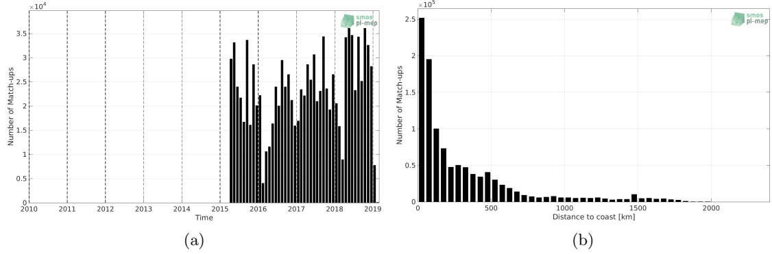
Figure 1: Number of match-ups between TSG (LEGOS-DM) and SMAP SSS L3 v4 - Monthly (RSS) SSS as a function of time (a) and as function of the distance to coast (b) over the North Atlantic Ocean Pi-MEP region and for the full satellite product period.
