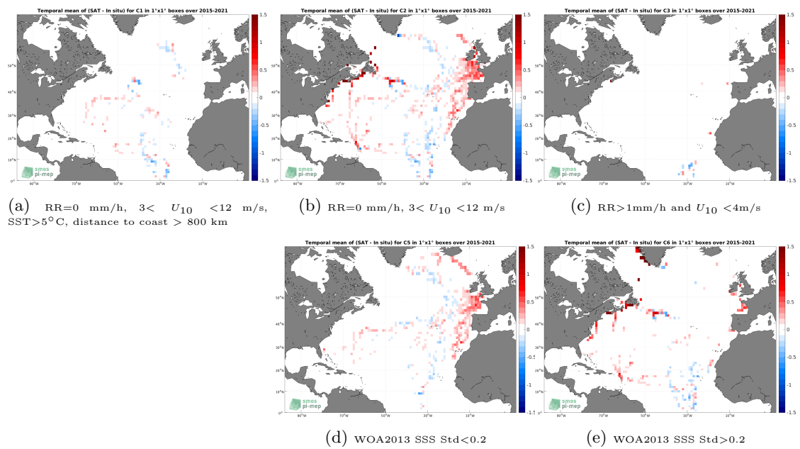
Figure 12: Temporal mean gridded over spatial boxes of size 1^\circ \times 1^\circ of \Delta\text{SSS} (SMAP SSS L3 v4 - Monthly (RSS) - TSG (GOSUD-Sailing-ship)) for 5 different subdatasets corresponding to:RR=0 mm/h, 3 < U_{10} < 12 m/s, SST >5^\circ\text{C} , distance to coast > 800 km (a), RR=0 mm/h, 3 < U_{10} < 12 m/s (b), RR >1 mm/h and U_{10} < 4 m/s (c), WOA2013 SSS Std <0.2 (d), WOA2013 SSS Std >0.2 (e).
