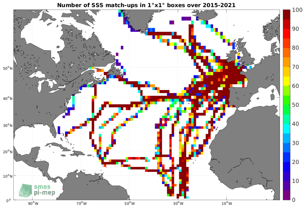
Figure 4: Number of SSS match-ups between TSG (GOSUD-Sailing-ship) SSS and the SMAP SSS L3 v4 - Monthly (RSS) SSS product for the North Atlantic Ocean Pi-MEP region over 1°x1° boxes and for the full satellite product period.
