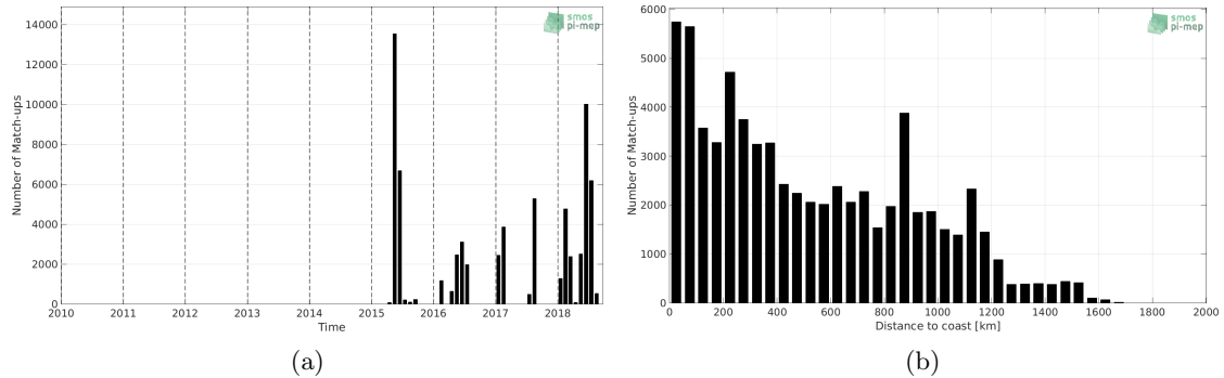
Figure 1: Number of match-ups between TSG (GOSUD-Sailing-ship) and SMAP SSS L3 v4 - Monthly (RSS) SSS as a function of time (a) and as function of the distance to coast (b) over the North Atlantic Ocean Pi-MEP region and for the full satellite product period.
