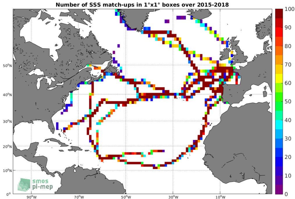
Figure 4: Number of SSS match-ups between TSG (GOSUD-Sailing-ship) SSS and the SMAP SSS L3 v4 - Monthly (RSS) SSS product for the North Atlantic Ocean Pi-MEP region over 1^\circ \times 1^\circ boxes and for the full satellite product period.
