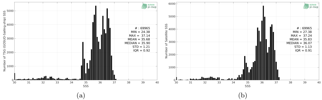
Figure 2: Histograms of SSS from TSG (GOSUD-Sailing-ship) (a) and SMAP SSS L3 v4 - Monthly (RSS) (b) considering all match-up pairs per bins of 0.1 over the North Atlantic Ocean Pi-MEP region and for the full satellite product period.
