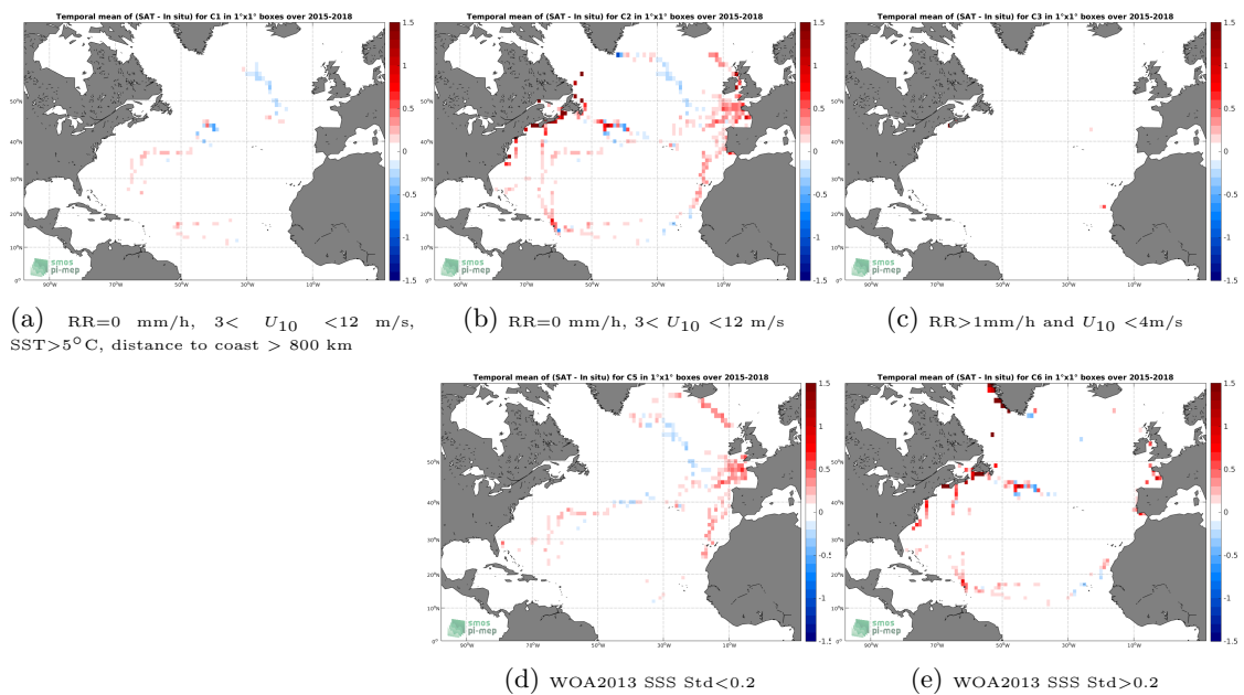
Figure 12: Temporal mean gridded over spatial boxes of size 1°x1° of \Delta SSS (SMAP SSS L3 v4 - Monthly (RSS) - TSG (GOSUD-Sailing-ship)) for 5 different subdatasets corresponding to:RR=0 mm/h, 3 < U_{10} < 12 m/s, SST>5°C, distance to coast > 800 km (a), RR=0 mm/h, 3 < U_{10} < 12 m/s (b), RR>1mm/h and U_{10} < 4 m/s (c), WOA2013 SSS Std<0.2 (d), WOA2013 SSS Std>0.2 (e).
