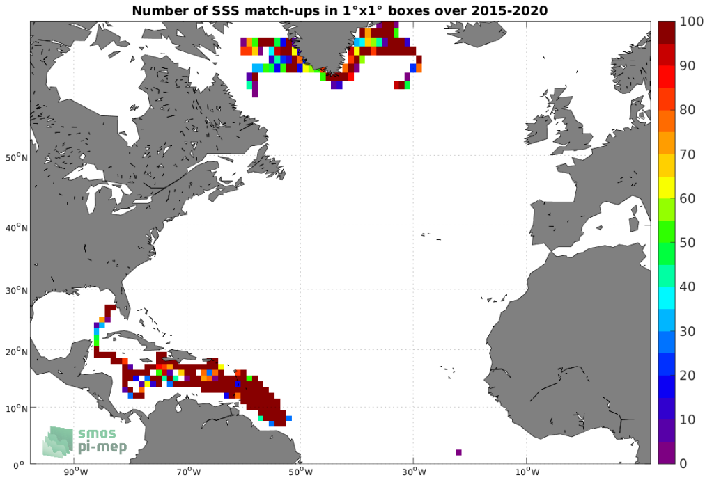
Figure 3: Number of SSS match-ups between Surface drifters SSS and the SMAP SSS L3 v4 - Monthly (RSS) SSS product for the North Atlantic Ocean Pi-MEP region over 1^\circ \times 1^\circ boxes and for the full satellite product period.
