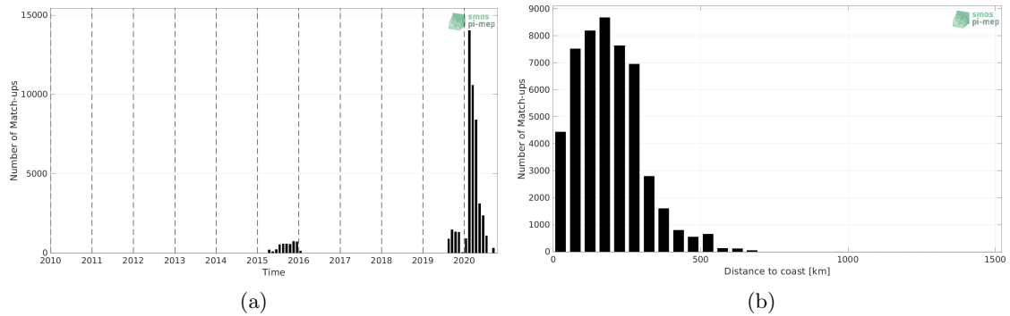
Figure 1: Number of match-ups between Surface drifters and SMAP SSS L3 v4 - Monthly (RSS) SSS as a function of time (a) and as function of the distance to coast (b) over the North Atlantic Ocean Pi-MEP region and for the full satellite product period.
