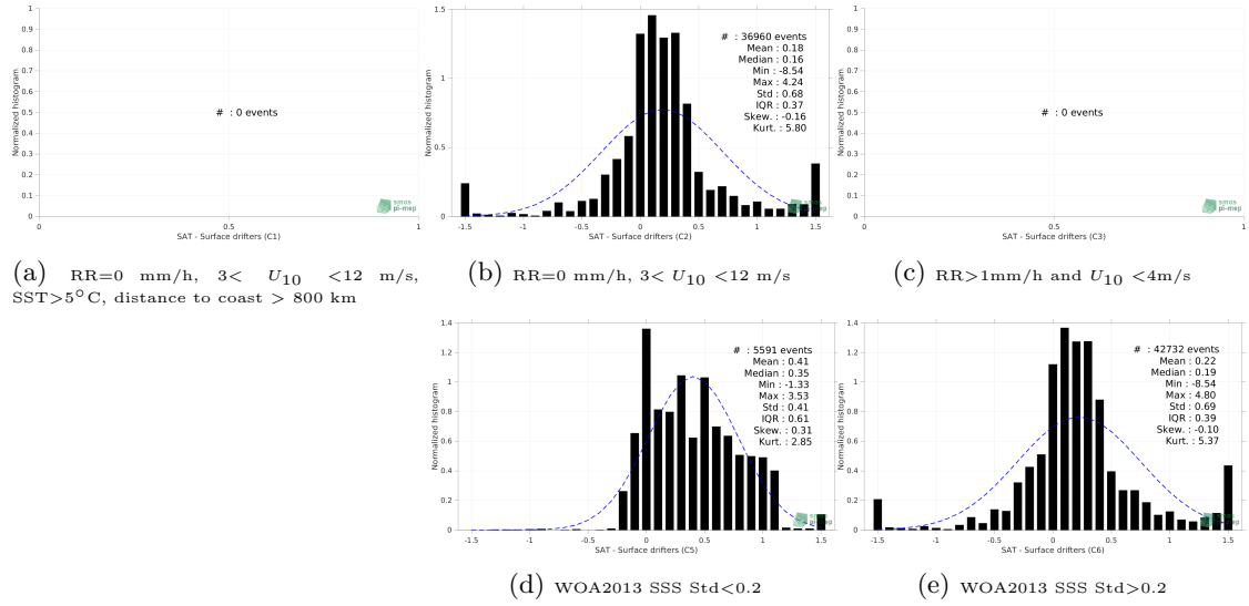
Figure 12: Normalized histogram of \Delta SSS (SMAP SSS L3 v4 - Monthly (RSS) - Surface drifters) for 5 different subdatasets corresponding to: RR=0 mm/h, 3 < U_{10} < 12 m/s, SST > 5°C, distance to coast > 800 km (a), RR=0 mm/h, 3 < U_{10} < 12 m/s (b), RR > 1mm/h and U_{10} < 4 m/s (c), WOA2013 SSS Std < 0.2 (d), WOA2013 SSS Std > 0.2 (e).
