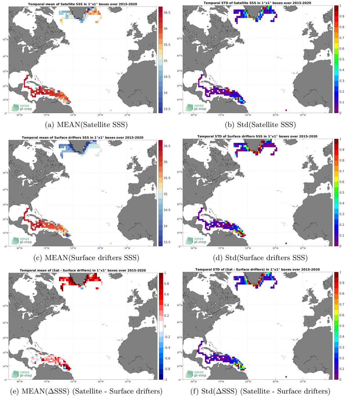
Figure 5: Temporal mean (left) and Std (right) of SSS from SMAP SSS L3 v4 - Monthly (RSS) (top), Surface drifters (middle), and of \Delta SSS (Satellite - Surface drifters). Only match-up pairs are used to generate these maps.
