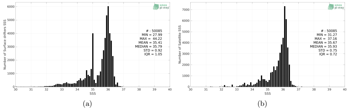
Figure 2: Histograms of SSS from Surface drifters (a) and SMAP SSS L3 v4 - Monthly (RSS) (b) considering all match-up pairs per bins of 0.1 over the North Atlantic Ocean Pi-MEP region and for the full satellite product period.
