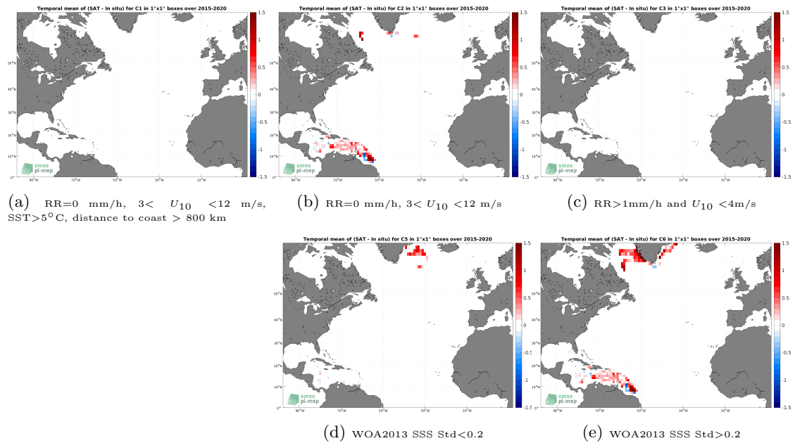
Figure 11: Temporal mean gridded over spatial boxes of size 1^\circ \times 1^\circ of \Delta SSS (SMAP SSS L3 v4 - Monthly (RSS) - Surface drifters) for 5 different subdatasets corresponding to:RR=0 mm/h, 3 < U_{10} < 12 m/s, SST >5^\circ\text{C} , distance to coast > 800 km (a), RR=0 mm/h, 3 < U_{10} < 12 m/s (b), RR >1 mm/h and U_{10} < 4 m/s (c), WOA2013 SSS Std <0.2 (d), WOA2013 SSS Std >0.2 (e).
