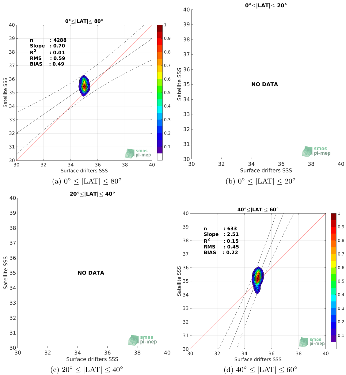
Figure 8: Contour maps of the concentration of SMAP SSS L3 v4 - Monthly (RSS) SSS (y-axis) versus Surface drifters SSS (x-axis) at match-up pairs for different latitude bands. For each plot, the red line shows x=y . The black thin and dashed lines indicate a linear fit through the data cloud and the \pm 95\% confidence levels, respectively. The number match-up pairs n , the slope and R^2 coefficient of the linear fit, the root mean square (RMS) and the mean bias between satellite and in situ data are indicated for each latitude band in each plots.
