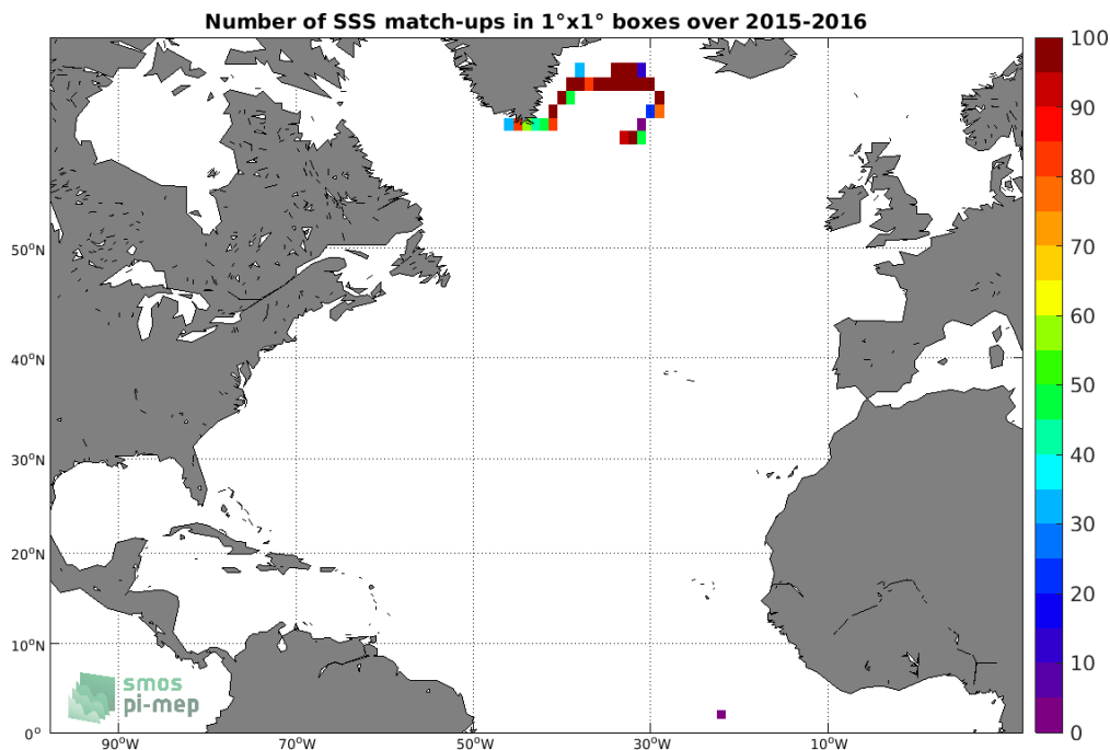
Figure 3: Number of SSS match-ups between Surface drifters SSS and the SMAP SSS L3 v4 - Monthly (RSS) SSS product for the North Atlantic Ocean Pi-MEP region over 1°x1° boxes and for the full satellite product period.
