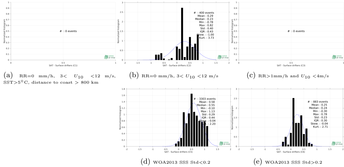
Figure 12: Normalized histogram of \Delta\text{SSS} (SMAP SSS L3 v4 - Monthly (RSS) - Surface drifters) for 5 different subdatasets corresponding to: RR=0 mm/h, 3 < U_{10} < 12 m/s, SST > 5^{\circ}\text{C} , distance to coast > 800 km (a), RR=0 mm/h, 3 < U_{10} < 12 m/s (b), RR > 1\text{mm/h} and U_{10} < 4\text{m/s} (c), WOA2013 SSS Std < 0.2 (d), WOA2013 SSS Std > 0.2 (e).
