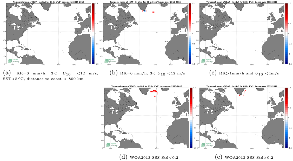
Figure 11: Temporal mean gridded over spatial boxes of size 1^{\circ}\times 1^{\circ} of \Delta\text{SSS} (SMAP SSS L3 v4 - Monthly (RSS) - Surface drifters) for 5 different subdatasets corresponding to:RR=0 mm/h, 3 < U_{10} < 12 m/s, SST >5^{\circ}\text{C} , distance to coast > 800 km (a), RR=0 mm/h, 3 < U_{10} < 12 m/s (b), RR >1 mm/h and U_{10} < 4 m/s (c), WOA2013 SSS Std <0.2 (d), WOA2013 SSS Std >0.2 (e).
