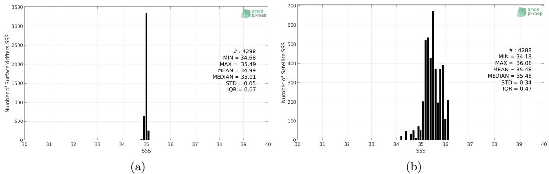
Figure 2: Histograms of SSS from Surface drifters (a) and SMAP-L3-RSS-V4-MONTHLY (b) considering all match-up pairs per bins of 0.1 over the North Atlantic Ocean Pi-MEP region and for the full satellite product period.
