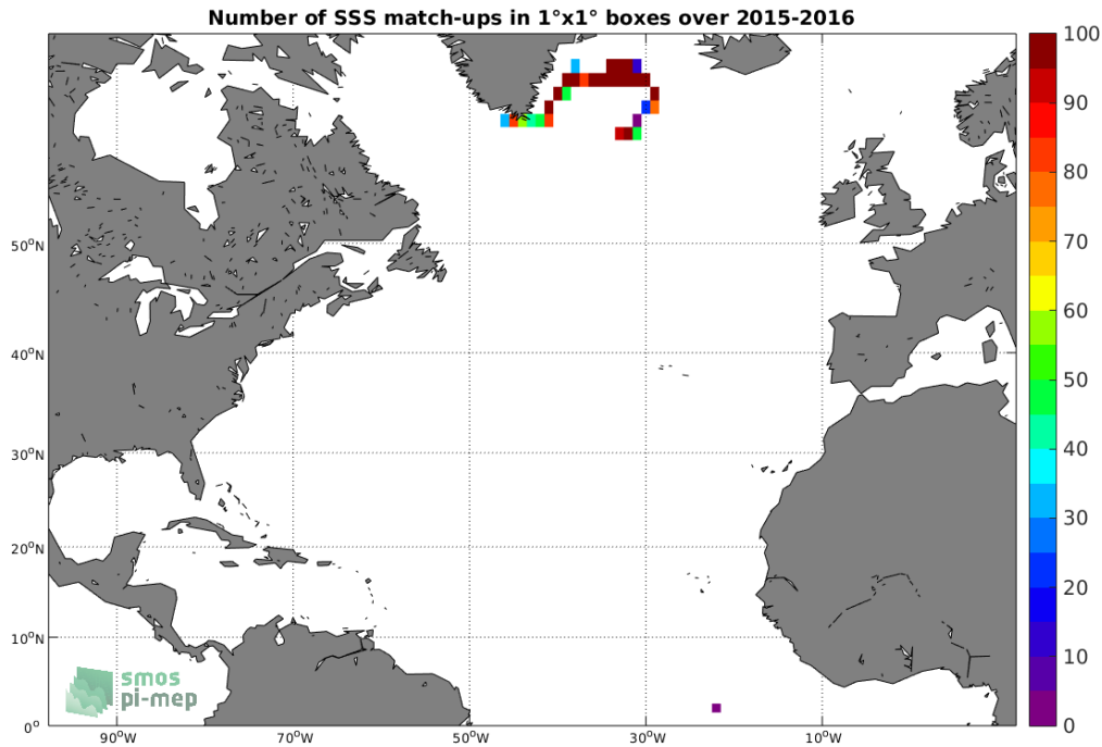
Figure 3: Number of SSS match-ups between Surface drifters SSS and the SMAP-L3-RSS-V4-MONTHLY SSS product for the North Atlantic Ocean Pi-MEP region over 1°x1° boxes and for the full satellite product period.
