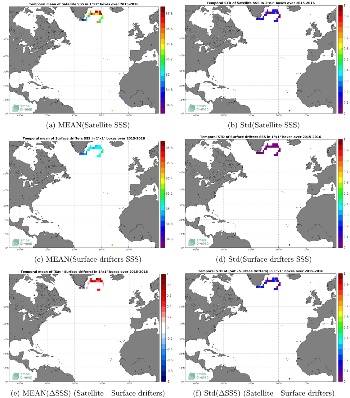
Figure 5: Temporal mean (left) and Std (right) of SSS from SMAP-L3-RSS-V4-MONTHLY (top), Surface drifters (middle), and of \Delta SSS (Satellite - Surface drifters). Only match-up pairs are used to generate these maps.
