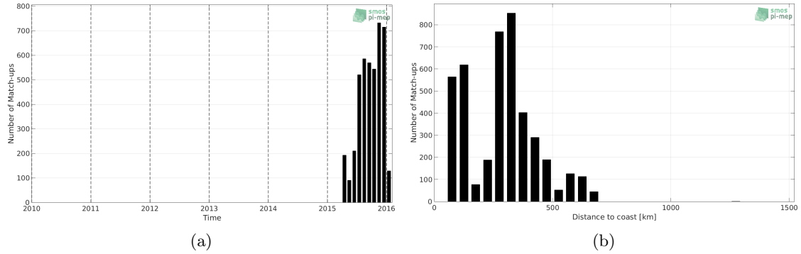
Figure 1: Number of match-ups between Surface drifters and SMAP-L3-RSS-V4-MONTHLY SSS as a function of time (a) and as function of the distance to coast (b) over the North Atlantic Ocean Pi-MEP region and for the full satellite product period.
