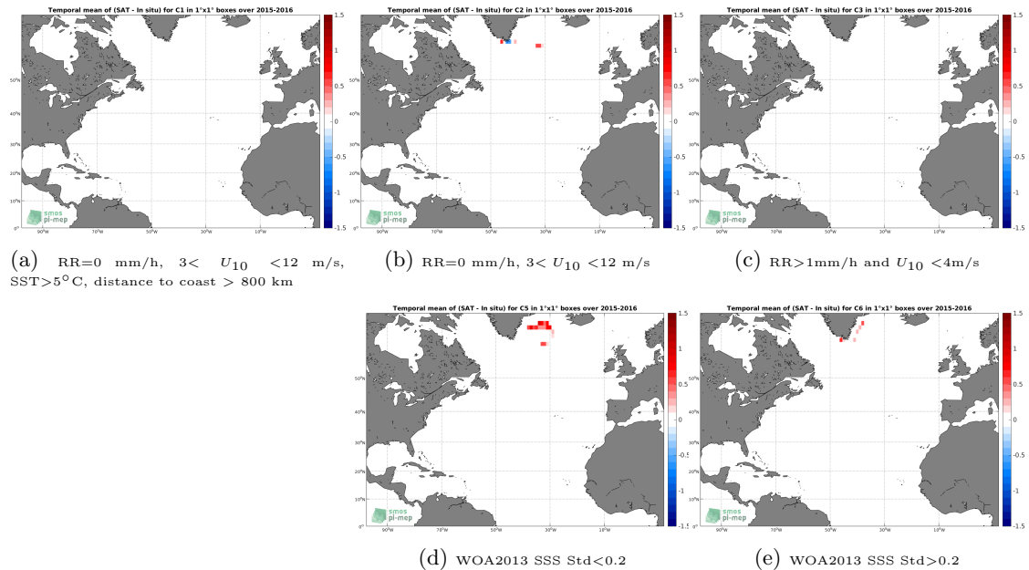
Figure 11: Temporal mean gridded over spatial boxes of size 1^{\circ}\times 1^{\circ} of \Delta\text{SSS} (SMAP-L3-RSS-V4-MONTHLY - Surface drifters) for 5 different subdatasets corresponding to:RR=0 mm/h, 3 < U_{10} < 12 m/s, SST > 5^{\circ}\text{C} , distance to coast > 800 km (a), RR=0 mm/h, 3 < U_{10} < 12 m/s (b), RR > 1 mm/h and U_{10} < 4 m/s (c), WOA2013 SSS Std < 0.2 (d), WOA2013 SSS Std > 0.2 (e).
