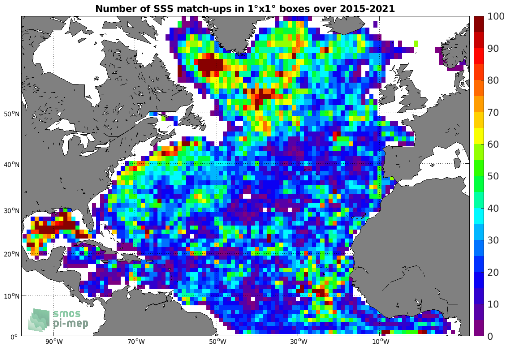
Figure 4: Number of SSS match-ups between Argo SSS and the SMAP SSS L3 v4 - Monthly (RSS) SSS product for the North Atlantic Ocean Pi-MEP region over 1^\circ \times 1^\circ boxes and for the full satellite product period.
