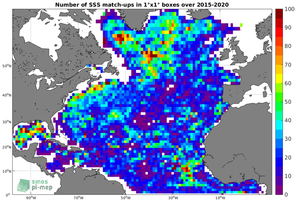
Figure 4: Number of SSS match-ups between Argos SSS and the SMAP-L3-RSS-V4-MONTHLY SSS product for the North Atlantic Ocean Pi-MEP region over 1°x1° boxes and for the full satellite product period.
