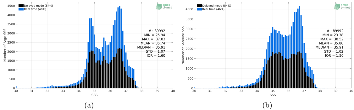
Figure 2: Histograms of SSS from Argo (a) and SMAP-L3-RSS-V4-MONTHLY (b) considering all match-up pairs per bins of 0.1 over the North Atlantic Ocean Pi-MEP region and for the full satellite product period.
