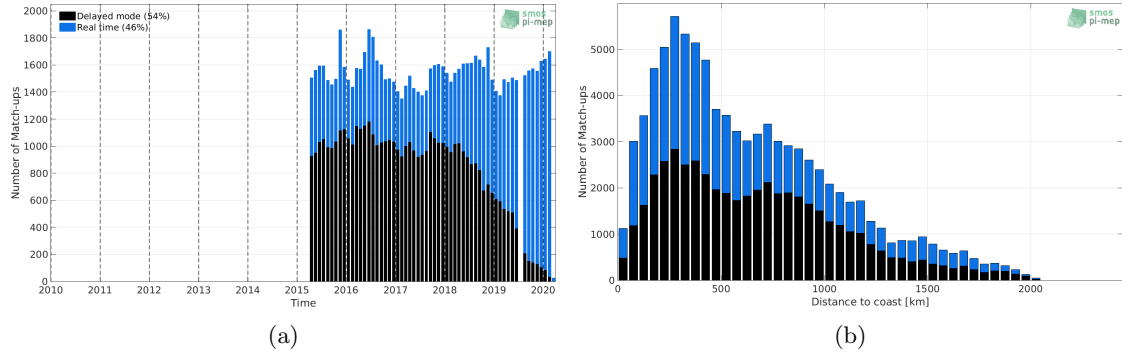
Figure 1: Number of match-ups between Argo and SMAP-L3-RSS-V4-MONTHLY SSS as a function of time (a) and as function of the distance to coast (b) over the North Atlantic Ocean Pi-MEP region and for the full satellite product period.
