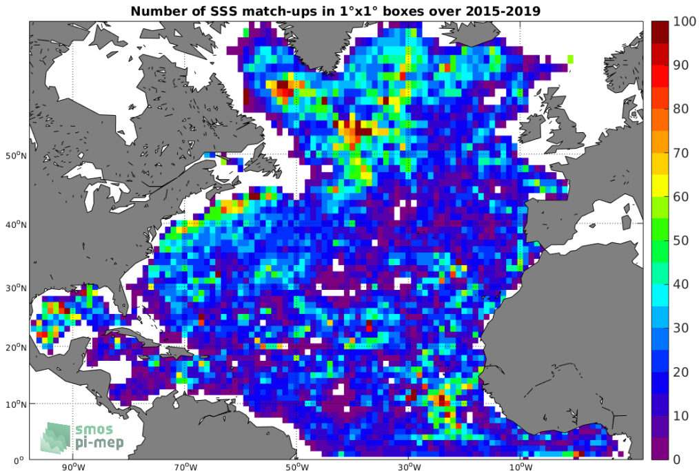
Figure 4: Number of SSS match-ups between Argo SSS and the SMAP-L3-RSS-V4-MONTHLY SSS product for the North Atlantic Ocean Pi-MEP region over 1°x1° boxes and for the full satellite product period.
