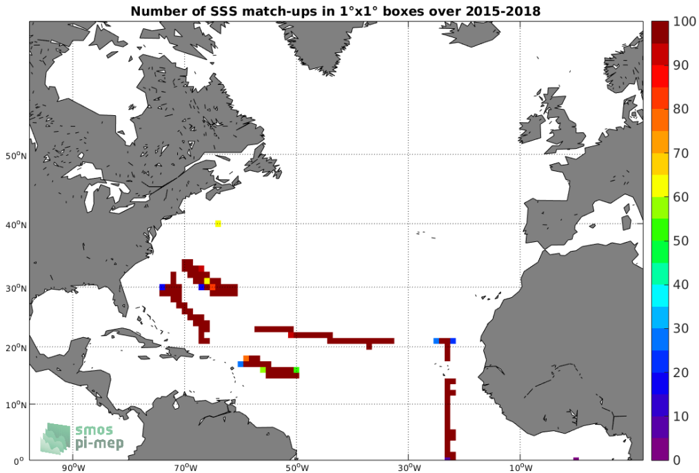
Figure 4: Number of SSS match-ups between TSG-SAMOS SSS and the SMAP-L3-RSS-V3-8DAY-RUNNING-70KM SSS product for the North Atlantic Ocean Pi-MEP region over 1^\circ \times 1^\circ boxes and for the full satellite product period.
