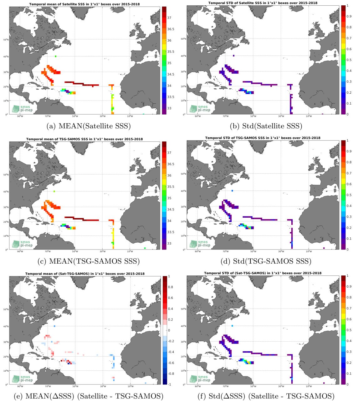
Figure 6: Temporal mean (left) and Std (right) of SSS from SMAP-L3-RSS-V3-8DAY-RUNNING-70KM (top), TSG-SAMOS (middle), and of \Delta SSS (Satellite - TSG-SAMOS). Only match-up pairs are used to generate these maps.
