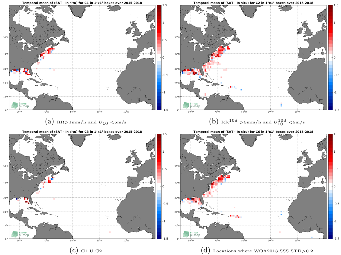
Figure 12: Temporal mean gridded over spatial boxes of size 1^\circ \times 1^\circ of \Delta SSS (SMAP-L3-RSS-V3-8DAY-RUNNING-70KM - TSG-SAMOS) for 4 different subdatasets corresponding to: RR > 1\text{mm/h} and U_{10} < 5\text{m/s} (a), RR^{10d} > 5\text{mm/h} and U_{10}^{10d} < 5\text{m/s} (b), C1 U C2 (c), Locations where WOA2013 SSS STD > 0.2 (d).
