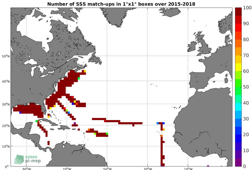
Figure 4: Number of SSS match-ups between TSG-SAMOS SSS and the SMAP-L3-RSS-V3-8DAY-RUNNING-70KM SSS product for the North Atlantic Ocean Pi-MEP region over 1°x1° boxes and for the full satellite product period.
