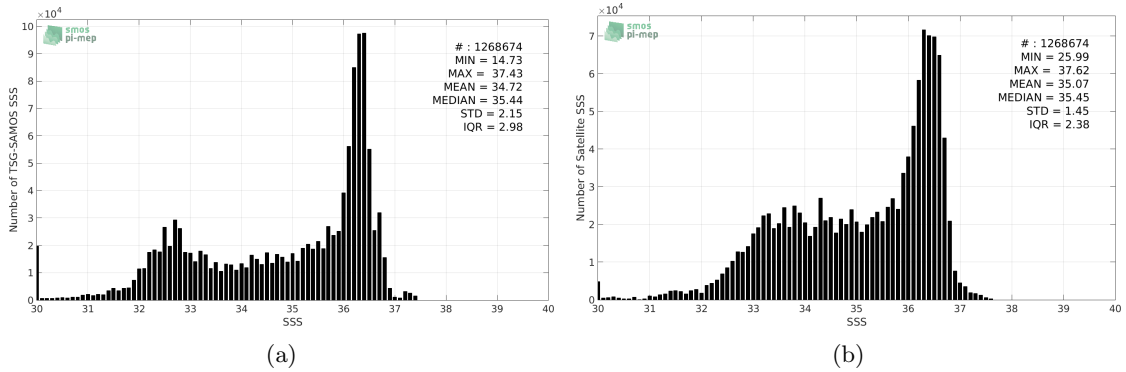
Figure 2: Histograms of SSS from TSG-SAMOS (a) and SMAP-L3-RSS-V3-8DAY-RUNNING-70KM (b) considering all match-up pairs per bins of 0.1 over the North Atlantic Ocean Pi-MEP region and for the full satellite product period.
