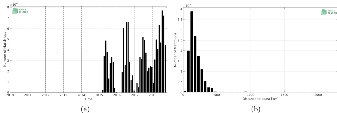
Figure 1: Number of match-ups between TSG-SAMOS and SMAP-L3-RSS-V3-8DAY-RUNNING-70KM SSS as a function of time (a) and as function of the distance to coast (b) over the North Atlantic Ocean Pi-MEP region and for the full satellite product period.
