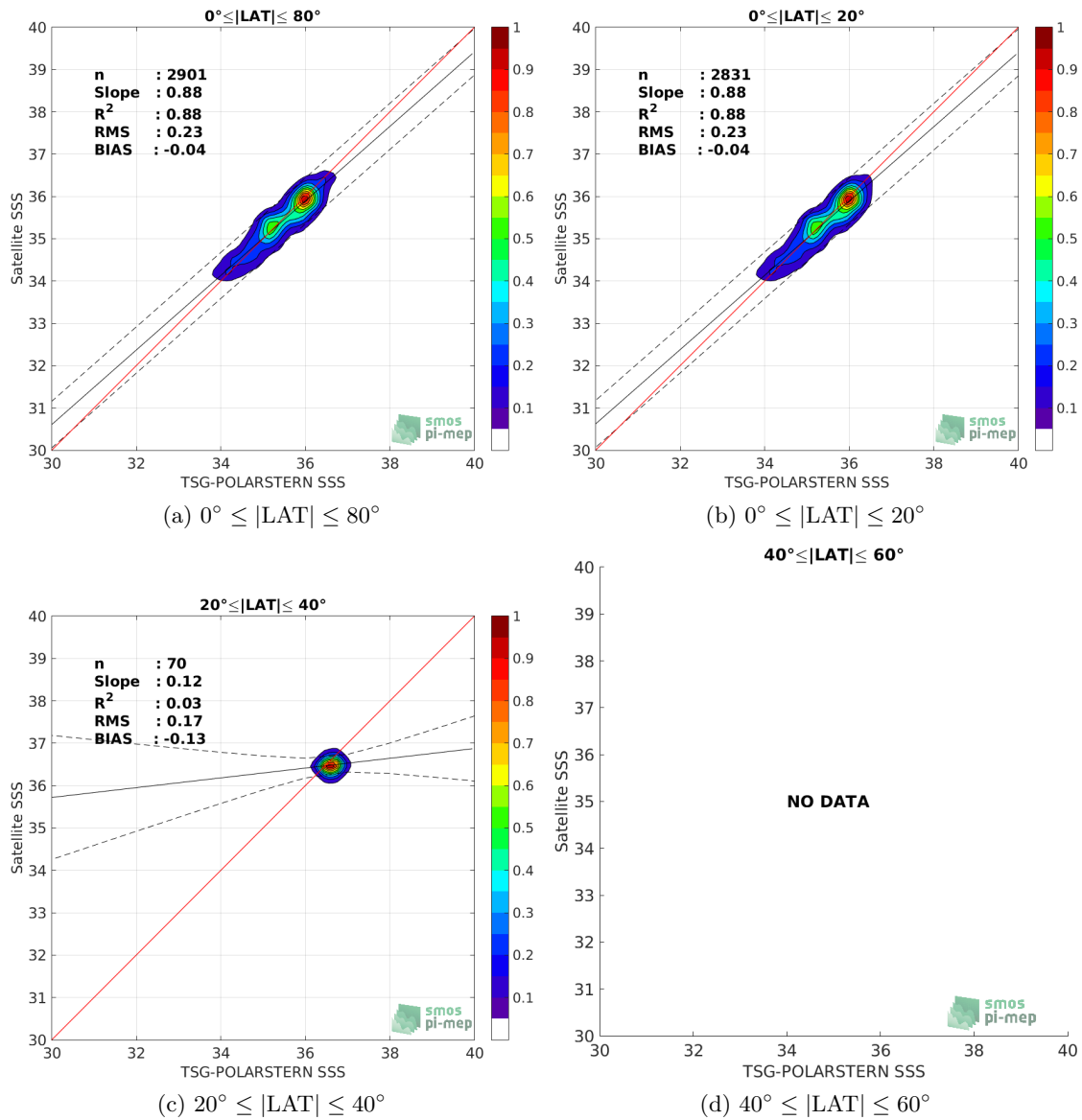
Figure 9: Contour maps of the concentration of SMAP-L3-RSS-V3-8DAY-RUNNING-70KM SSS (y-axis) versus TSG-POLARSTERN SSS (x-axis) at match-up pairs for different latitude bands. For each plot, the red line shows x=y . The black thin and dashed lines indicate a linear fit through the data cloud and the \pm 95\% confidence levels, respectively. The number match-up pairs n , the slope and R^2 coefficient of the linear fit, the root mean square (RMS) and the mean bias between satellite and in situ data are indicated for each latitude band in each plots.
