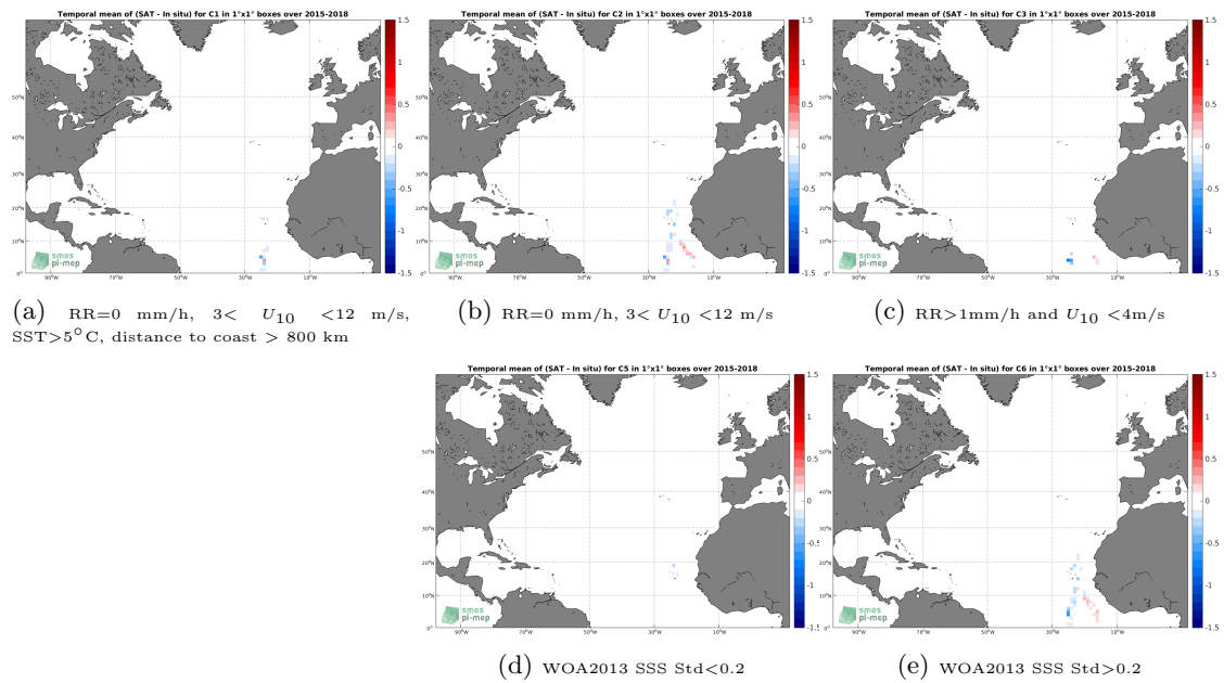
Figure 12: Temporal mean gridded over spatial boxes of size 1^\circ \times 1^\circ of \Delta SSS (SMAP-L3-RSS-V3-8DAY-RUNNING-70KM - TSG-POLARSTERN) for 5 different subdatasets corresponding to: RR=0 mm/h, 3 < U_{10} < 12 m/s, SST > 5^\circ\text{C} , distance to coast > 800 km (a), RR=0 mm/h, 3 < U_{10} < 12 m/s (b), RR > 1 mm/h and U_{10} < 4 m/s (c), WOA2013 SSS Std < 0.2 (d), WOA2013 SSS Std > 0.2 (e).
