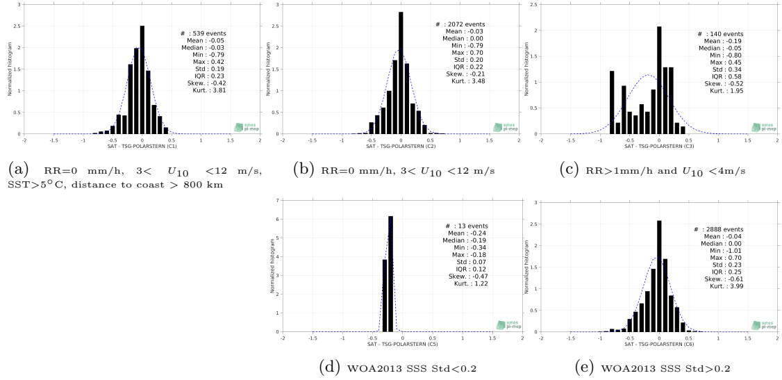
Figure 13: Normalized histogram of \Delta SSS (SMAP-L3-RSS-V3-8DAY-RUNNING-70KM - TSG-POLARSTERN) for 5 different subdatasets corresponding to: RR=0 mm/h, 3 < U_{10} < 12 m/s, SST>5°C, distance to coast > 800 km (a), RR=0 mm/h, 3 < U_{10} < 12 m/s (b), RR>1mm/h and U_{10} < 4 m/s (c), WOA2013 SSS Std<0.2 (d), WOA2013 SSS Std>0.2 (e).
