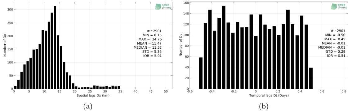
Figure 5: Histograms of the spatial (a) and temporal (b) lags between the time of the TSG-POLARSTERN measurements and the date of the corresponding SMAP-L3-RSS-V3-8DAY-RUNNING-70KM SSS product.
