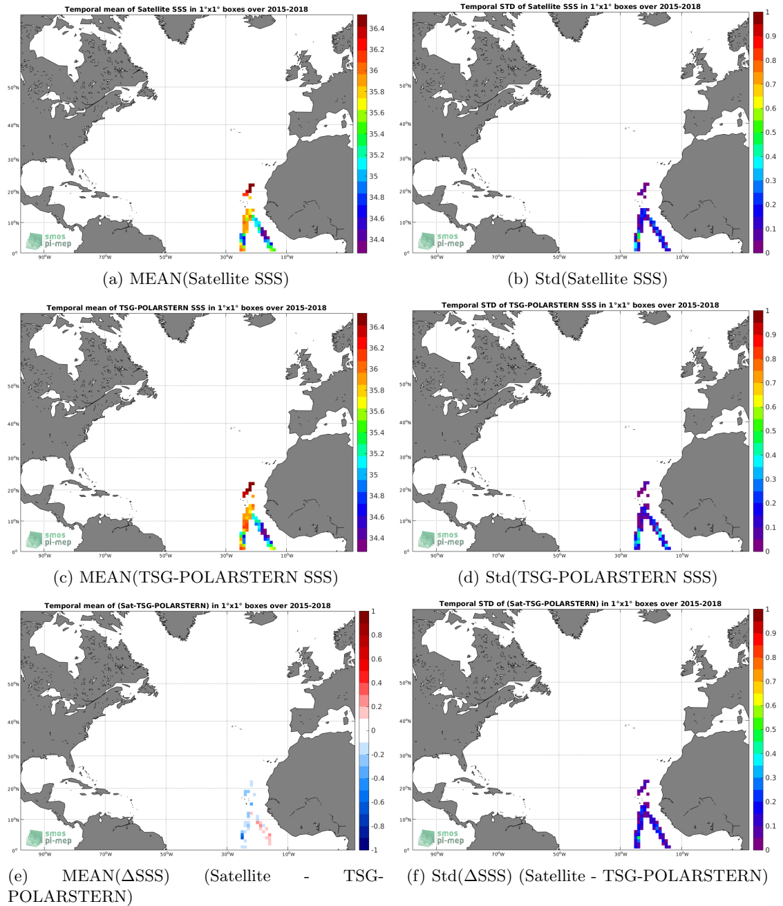
Figure 6: Temporal mean (left) and Std (right) of SSS from SMAP-L3-RSS-V3-8DAY-RUNNING-70KM (top), TSG-POLARSTERN (middle), and of \Delta SSS (Satellite - TSG-POLARSTERN). Only match-up pairs are used to generate these maps.
