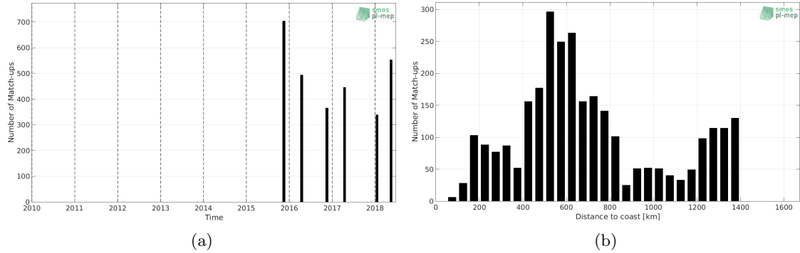
Figure 1: Number of match-ups between TSG-POLARSTERN and SMAP-L3-RSS-V3-8DAY-RUNNING-70KM SSS as a function of time (a) and as function of the distance to coast (b) over the North Atlantic Ocean Pi-MEP region and for the full satellite product period.
