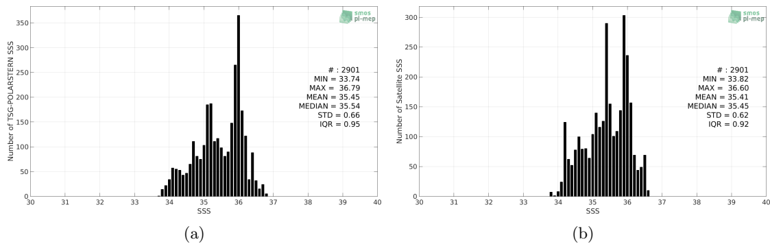
Figure 2: Histograms of SSS from TSG-POLARSTERN (a) and SMAP-L3-RSS-V3-8DAY-RUNNING-70KM (b) considering all match-up pairs per bins of 0.1 over the North Atlantic Ocean Pi-MEP region and for the full satellite product period.
