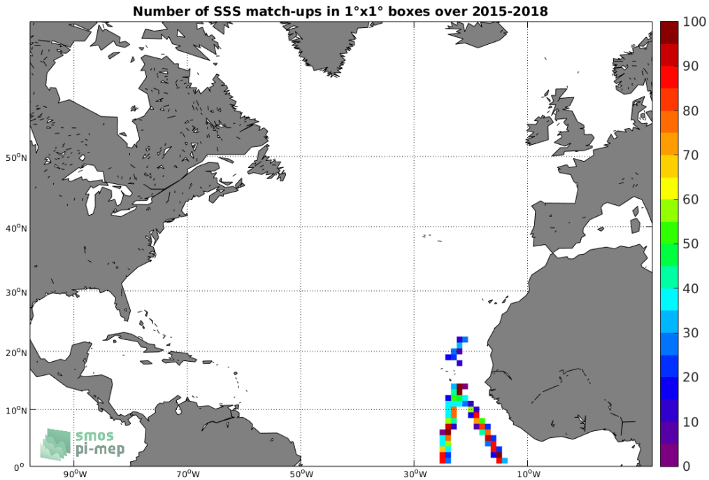
Figure 4: Number of SSS match-ups between TSG-POLARSTERN SSS and the SMAP-L3-RSS-V3-8DAY-RUNNING-70KM SSS product for the North Atlantic Ocean Pi-MEP region over 1°x1° boxes and for the full satellite product period.
