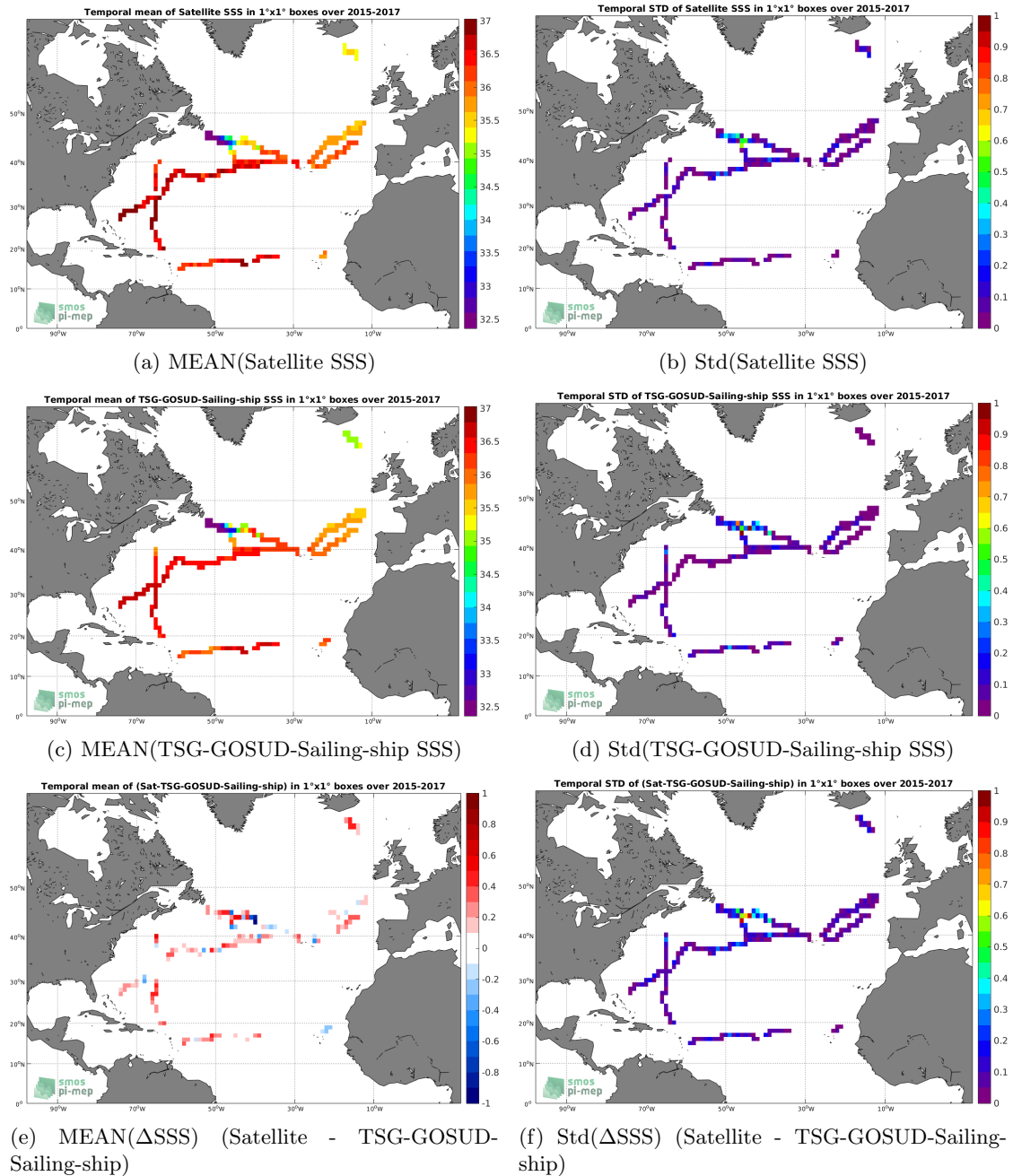
Figure 6: Temporal mean (left) and Std (right) of SSS from SMAP-L3-RSS-V3-8DAY-RUNNING-70KM (top), TSG-GOSUD-Sailing-ship (middle), and of \Delta SSS (Satellite - TSG-GOSUD-Sailing-ship). Only match-up pairs are used to generate these maps.
