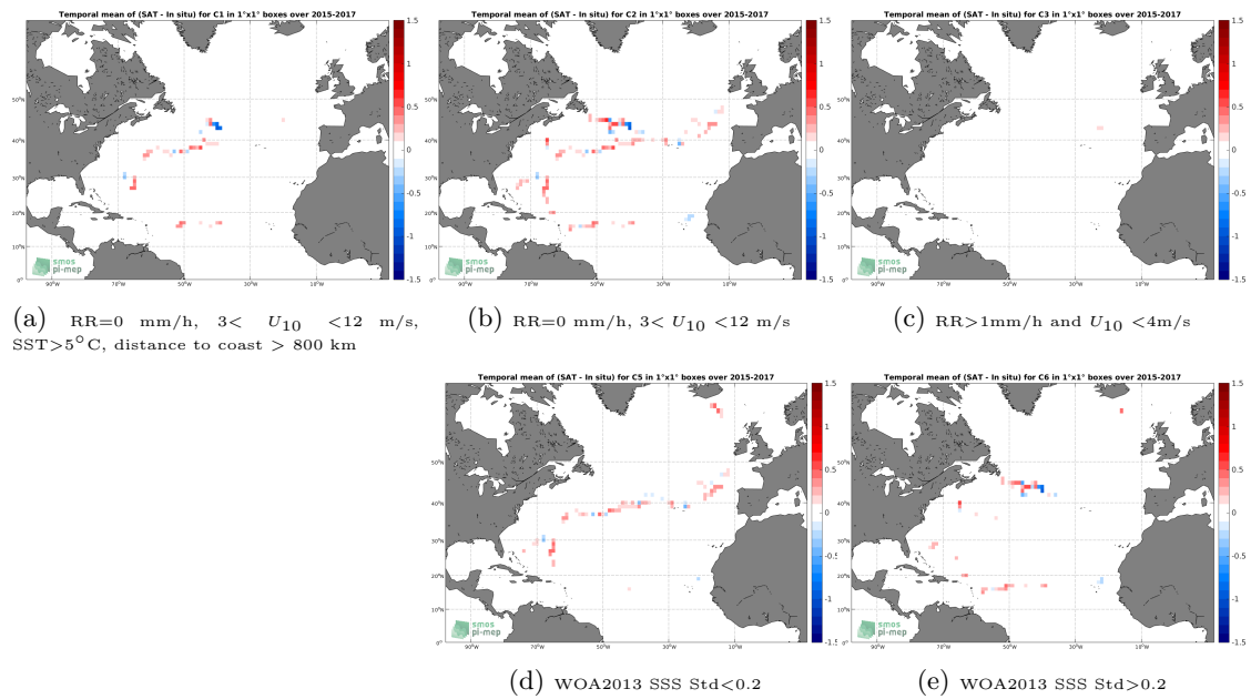
Figure 12: Temporal mean gridded over spatial boxes of size 1^\circ \times 1^\circ of \Delta SSS (SMAP-L3-RSS-V3-8DAY-RUNNING-70KM - TSG-GOSUD-Sailing-ship) for 5 different subdatasets corresponding to:RR=0 mm/h, 3 < U_{10} < 12 m/s, SST > 5^\circ C, distance to coast > 800 km (a), RR=0 mm/h, 3 < U_{10} < 12 m/s (b), RR > 1 mm/h and U_{10} < 4 m/s (c), WOA2013 SSS Std < 0.2 (d), WOA2013 SSS Std > 0.2 (e).
