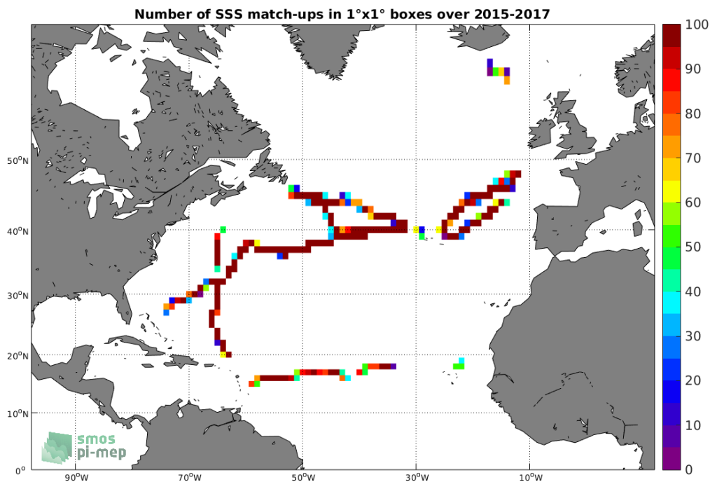
Figure 4: Number of SSS match-ups between TSG-GOSUD-Sailing-ship SSS and the SMAP-L3-RSS-V3-8DAY-RUNNING-70KM SSS product for the North Atlantic Ocean Pi-MEP region over 1^\circ \times 1^\circ boxes and for the full satellite product period.
