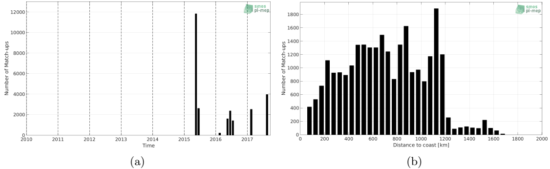
Figure 1: Number of match-ups between TSG-GOSUD-Sailing-ship and SMAP-L3-RSS-V3-8DAY-RUNNING-70KM SSS as a function of time (a) and as function of the distance to coast (b) over the North Atlantic Ocean Pi-MEP region and for the full satellite product period.
