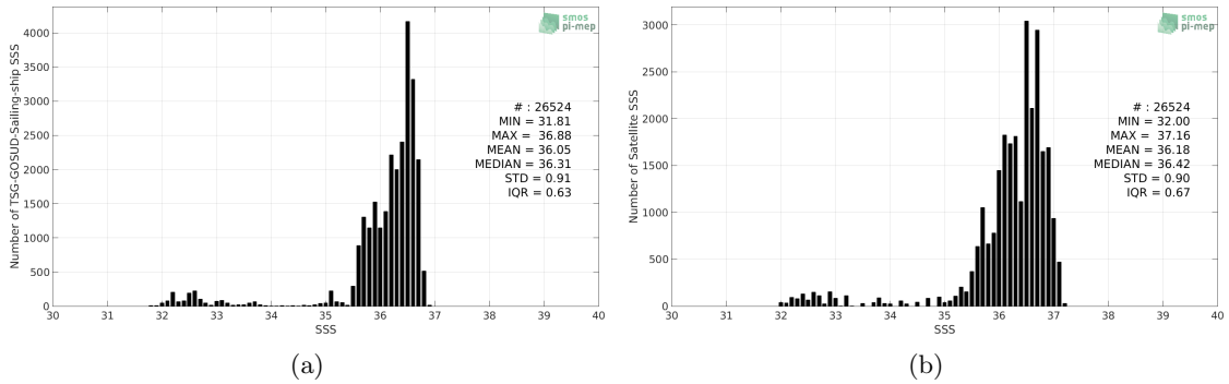
Figure 2: Histograms of SSS from TSG-GOSUD-Sailing-ship (a) and SMAP-L3-RSS-V3-8DAY-RUNNING-70KM (b) considering all match-up pairs per bins of 0.1 over the North Atlantic Ocean Pi-MEP region and for the full satellite product period.
