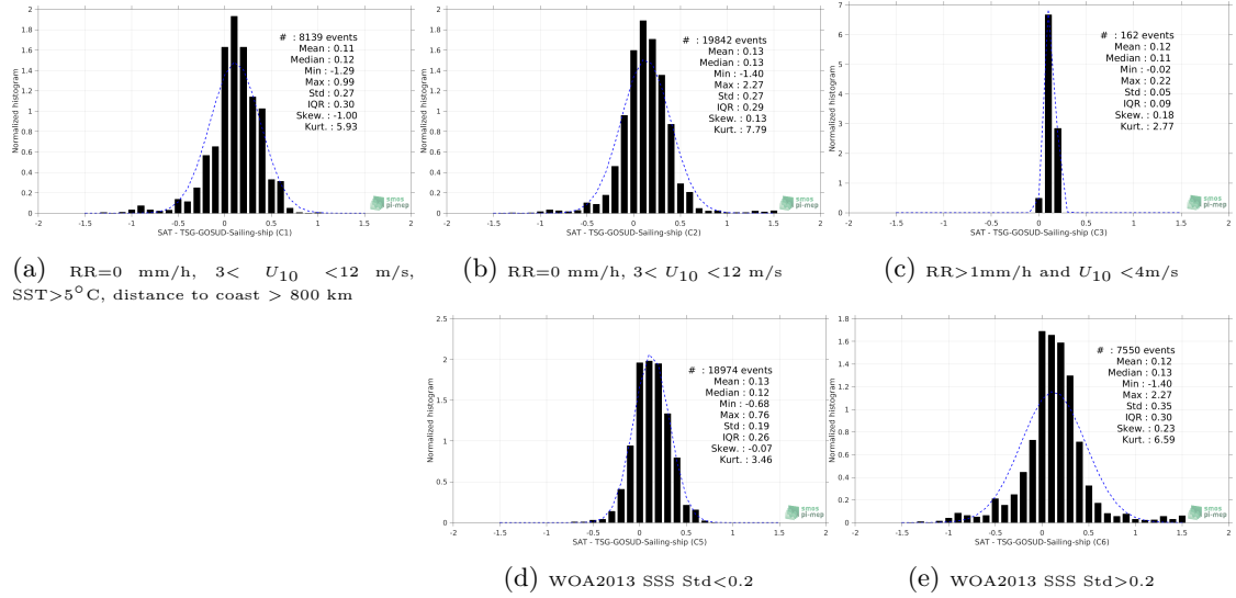
Figure 13: Normalized histogram of \Delta\text{SSS} (SMAP-L3-RSS-V3-8DAY-RUNNING-70KM - TSG-GOSUD-Sailing-ship) for 5 different subdatasets corresponding to: RR=0 mm/h, 3 < U_{10} < 12 m/s, SST > 5^{\circ}\text{C} , distance to coast > 800 km (a), RR=0 mm/h, 3 < U_{10} < 12 m/s (b), RR > 1\text{mm/h} and U_{10} < 4\text{m/s} (c), WOA2013 SSS Std < 0.2 (d), WOA2013 SSS Std > 0.2 (e).
