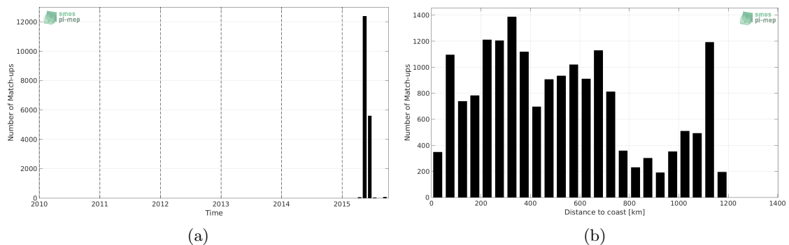
Figure 1: Number of match-ups between TSG-GOSUD-Sailing-ship and SMAP-L3-RSS-V3-8DAY-RUNNING-70KM SSS as a function of time (a) and as function of the distance to coast (b) over the North Atlantic Ocean Pi-MEP region and for the full satellite product period.
