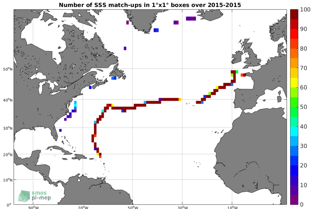
Figure 4: Number of SSS match-ups between TSG-GOSUD-Sailing-ship SSS and the SMAP-L3-RSS-V3-8DAY-RUNNING-70KM SSS product for the North Atlantic Ocean Pi-MEP region over 1°x1° boxes and for the full satellite product period.
