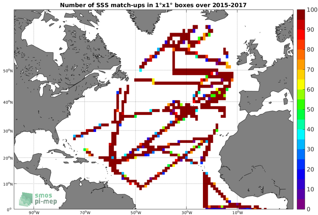
Figure 4: Number of SSS match-ups between TSG-GOSUD-Research-vessel SSS and the SMAP-L3-RSS-V3-8DAY-RUNNING-70KM SSS product for the North Atlantic Ocean Pi-MEP region over 1^\circ \times 1^\circ boxes and for the full satellite product period.
